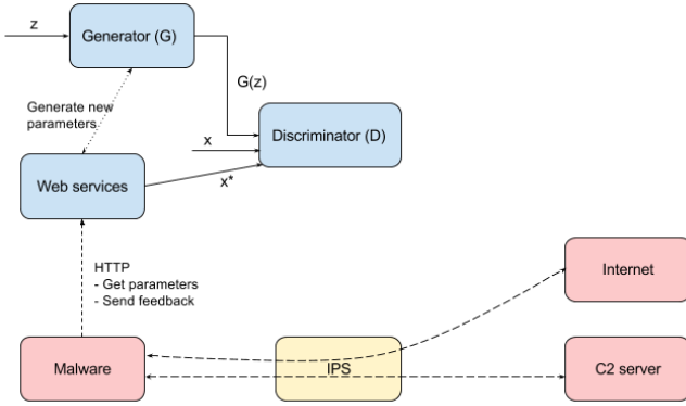
Fig. 1. Network experiments setup. The GAN is implemented independently and communicates with the malware through a web service. The malware gets the parameters and modifies its traffic in real time. The C2 channel should be maintained and should be operational. The IPS blocks all the traffic that does not look like Facebook chat.
