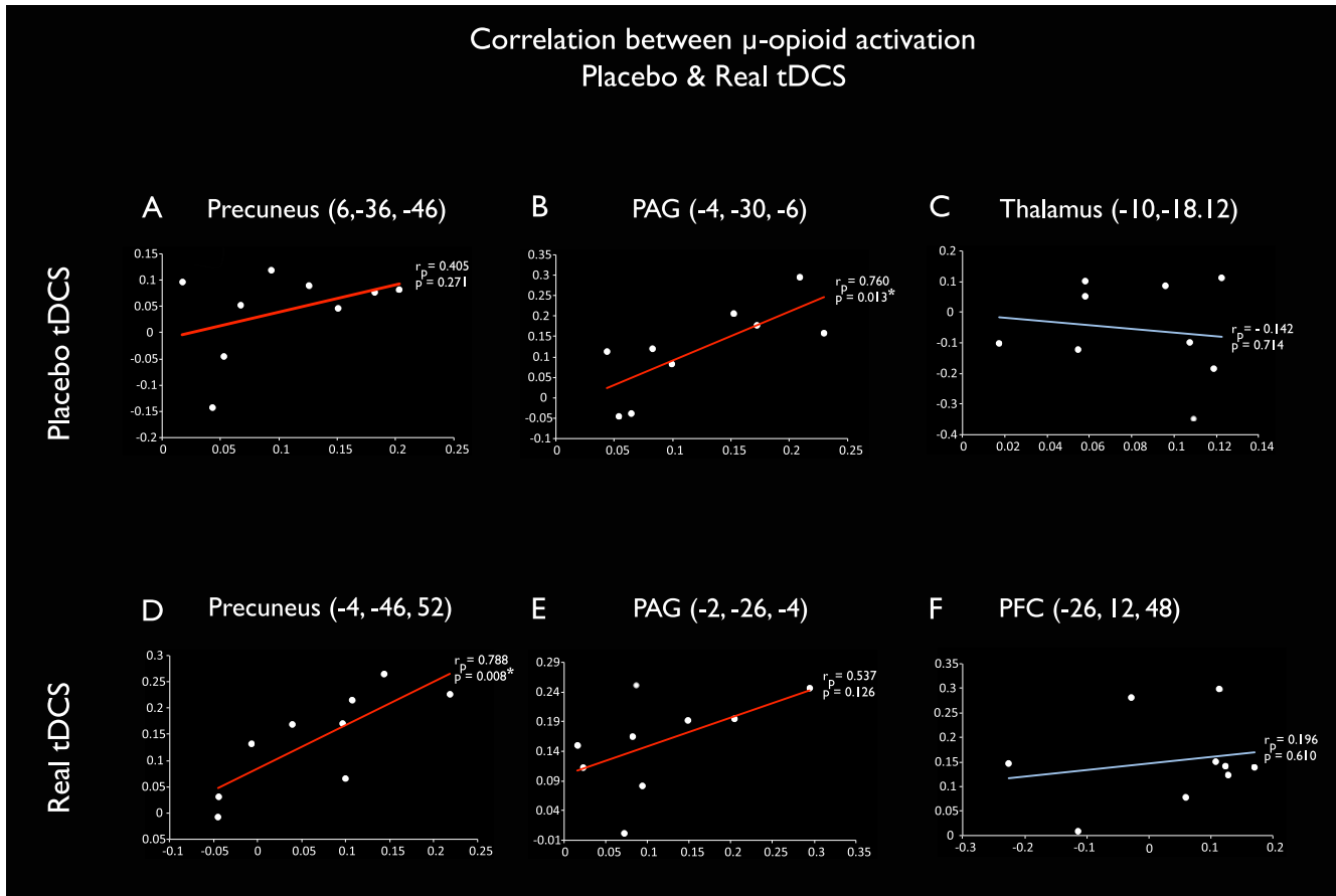
Figure 3. Correlation between placebo and real tDCS-induced MOR activation. MOR BP_{ND} during placebo (x axis) and real (y axis) tDCS for each subject in the clusters of \mu -opioid activation induced by placebo (A–C) and real (D–F) tDCS. The same clusters are illustrated in the figure 2. Positive correlations can be observed in precuneus and PAG (red lines) but not in thalamus and PFC (blue lines). Statistically significant values at p < 0.05 were found in the PAG cluster activated during placebo tDCS ( r_p = 0.760 , p = 0.013 , 3B) and in the precuneus cluster activated during active tDCS ( r_p = 0.788 , p = 0.008 , 3D).
