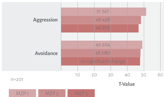
Fig. 4: Graphical representation of the assessment of the affected »unspecific stress management measures« at the times of the three measurements (during MZP 2 significantly).
