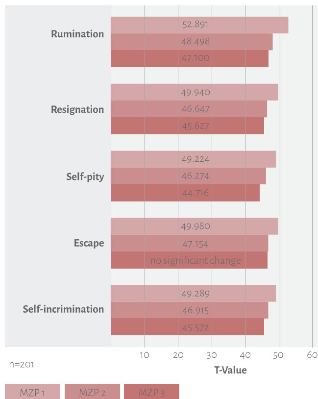
Fig. 3: Graphical representation of the assessment of the affected »negative stress management measures« during the three times of measurement (during MZP 2 significantly).
