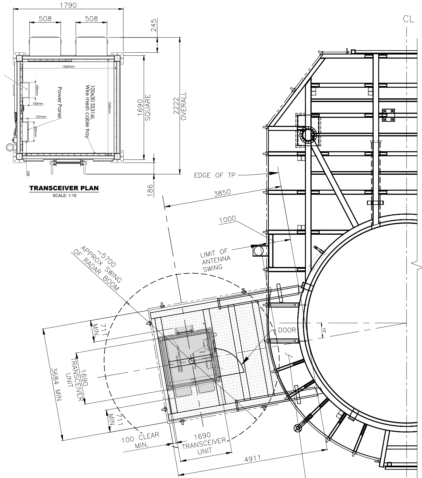
EXTERNAL PLATFORM RADAR/ANTENNA FRAMING PLAN - LOCATION II SCALE: 1:30
