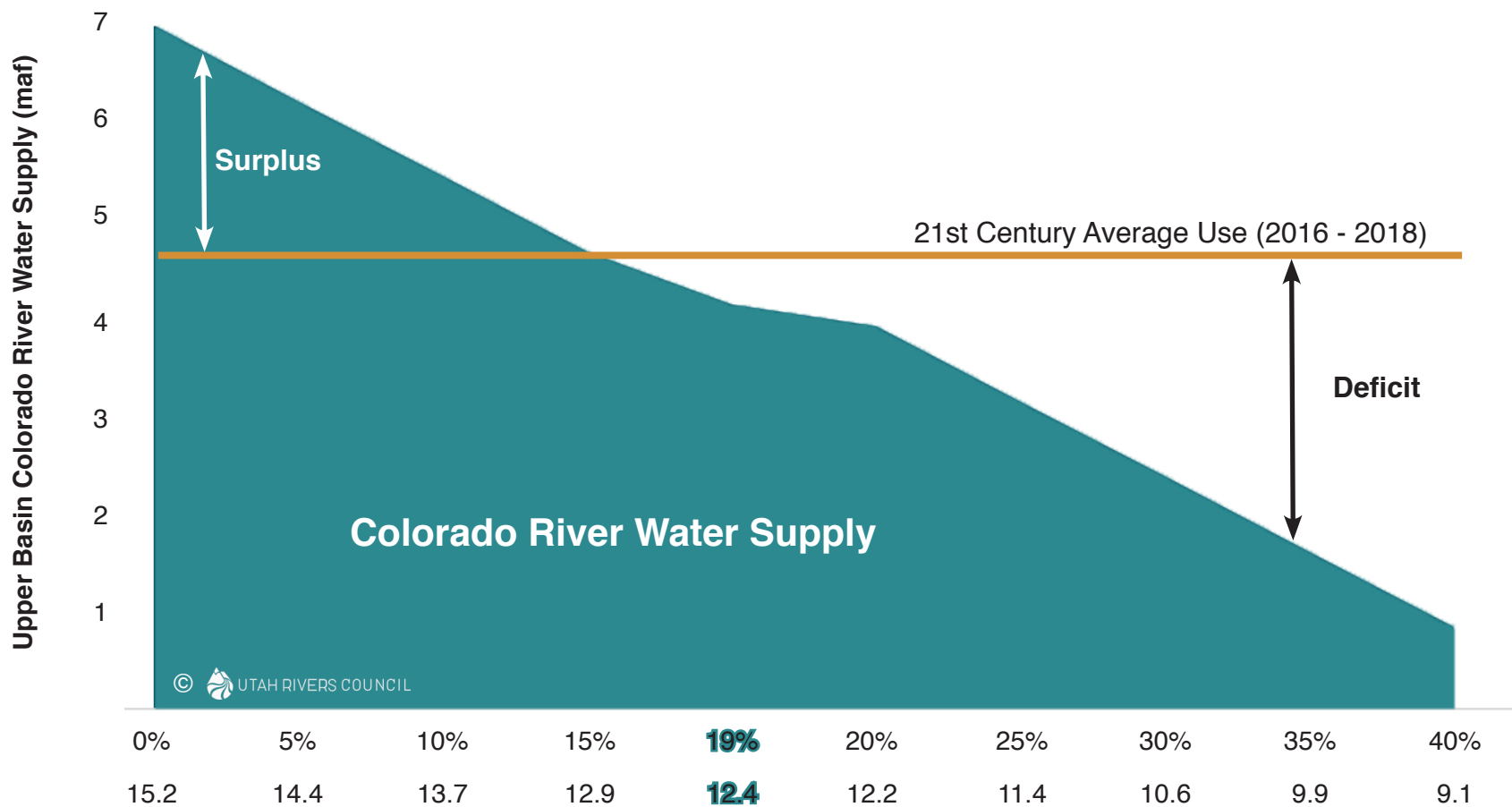
Figure 7. Declining Upper Basin Water Supply vs. Current Water Use
