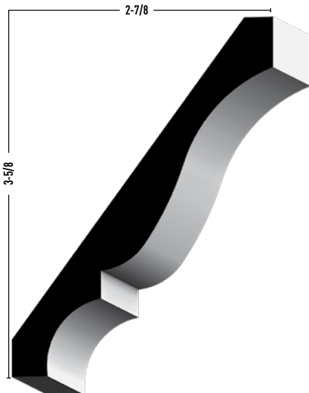
L 47 19/32 x 4-5/8 MDF 16' 9/16 x 4-5/8 PRIMED 16' PINE 16'
