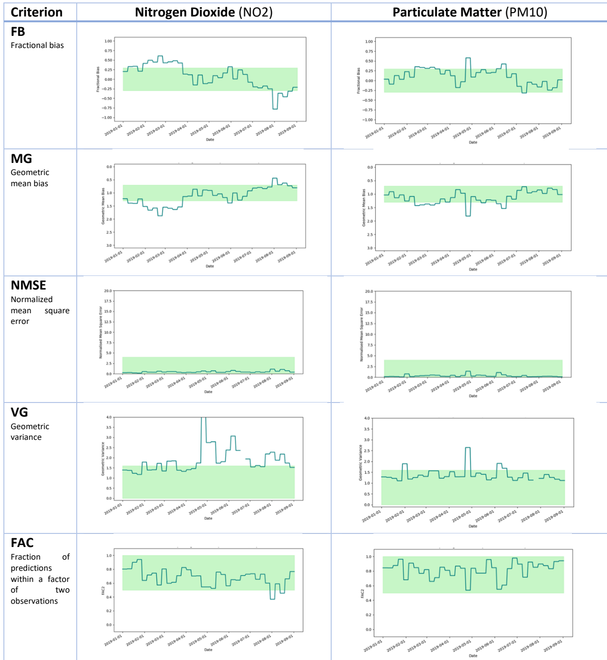
Figure 6: Performance of eLichens model each week over 7 months
