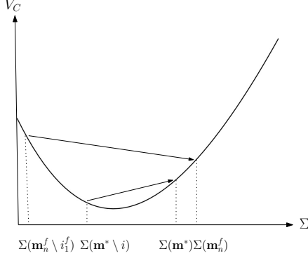
Figure 4: Any citizen i \in \mathbf{m}^* has strictly lower marginal informativeness than passive citizen i_1^f \in \mathbf{m}_n^f .
