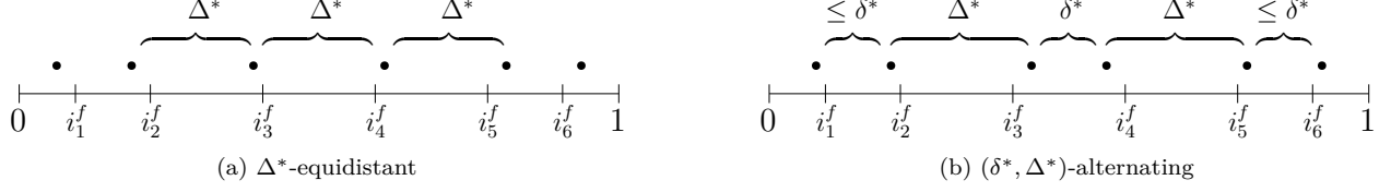
Figure 7: Optimal patterns of distortions in Proposition 4.3.
