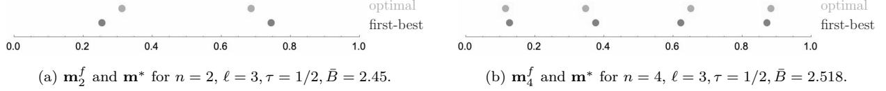
Figure 6: Distortions in small minipublics.
