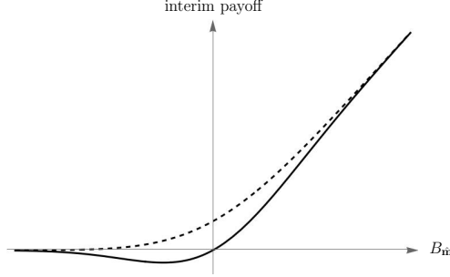
Figure 1: The citizen's interim payoff B_{\hat{m}}\Phi(B_{\hat{m}}/\tau) (solid line) and the policymaker's expected payoff B_{\hat{m}}\Phi(B_{\hat{m}}/\tau) + \tau\phi(B_{\hat{m}}/\tau) (dashed line) for every realized post-minipublic value B_{\hat{m}} .
