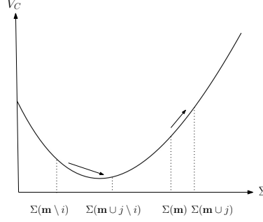
Figure 3: No distortion in minipublic size: citizens i \in \mathbf{m} and j \notin \mathbf{m} prefer to be active in \mathbf{m} \cup \{j\} if \mathbf{m} is active.
