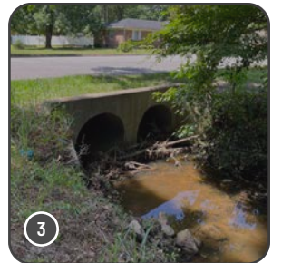
Burkhead Street: Existing Culvert Condition
