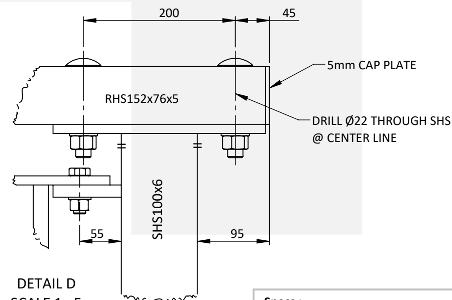
END POST
