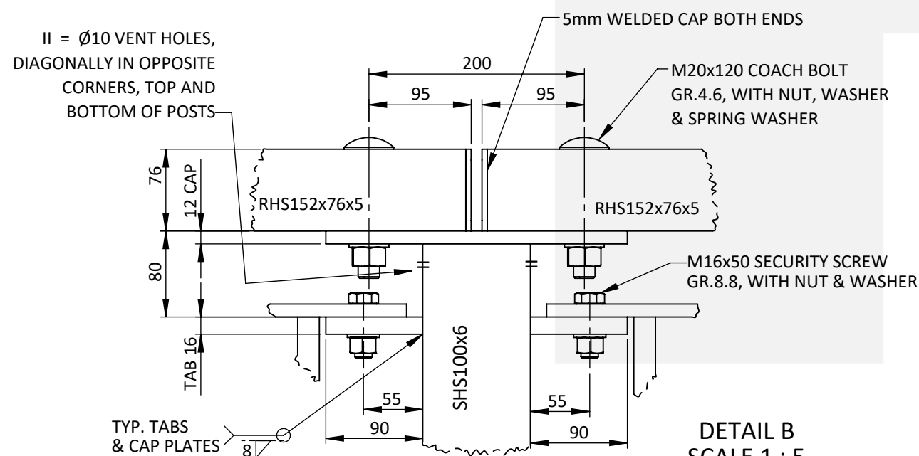
INTERMEDIATE POST
