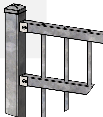
Bracket Detail
