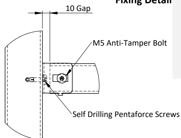
Fixing Detail
