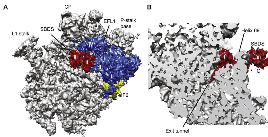
Fig. 3. SBDS and EFL1 proofread the structural and functional integrity of the nascent 60S subunit. (A) Crown view and (B) transverse section of the cryo-EM maps of the 60S-eIF6-SBDS-EFL1 complex. The 60S subunit is coloured grey, SBDS is red, EFL1 is blue and eIF6 is yellow. SBDS domains II and III and EFL1 domains I–V are shown. CP, central protuberance.
