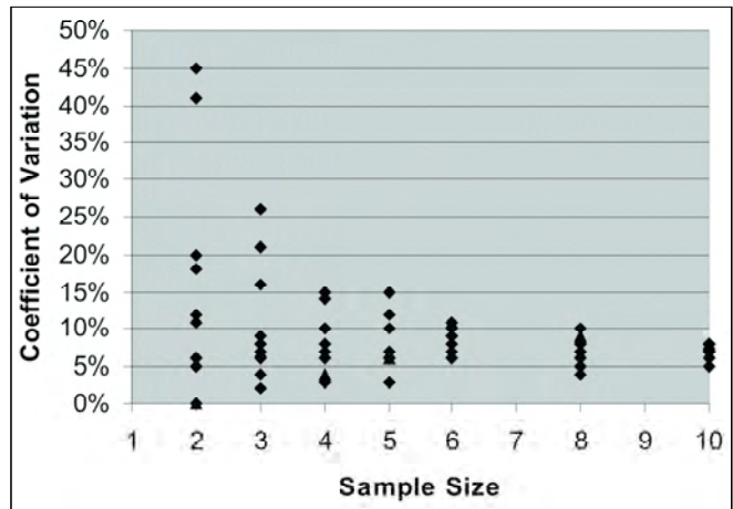
Figure 2. Sensitivity analysis to assess implications of sample size (e.g., number of clusters) on the coefficient of variation for density of large trees ( \geq 24 inches dbh) based on pilot data from White River NWR.
