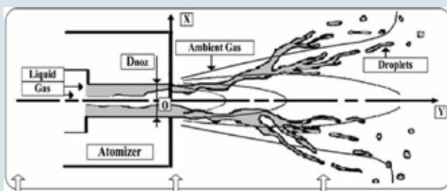
FIGURE 11. EXPLODING ANNULAR FLOW TECHNOLOGY.
