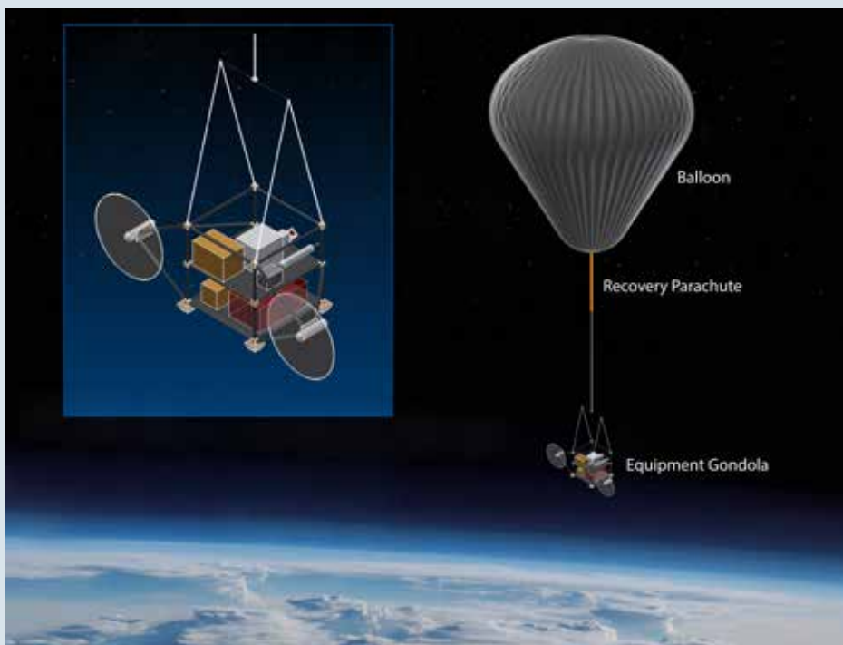
FIGURE 9. STRATOSPHERIC CONTROLLED PERTURBATION EXPERIMENT (SCOPEX).
