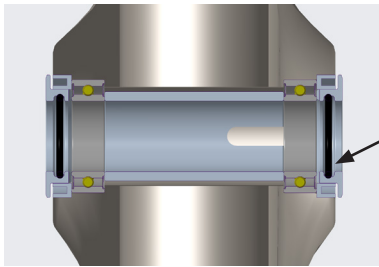
Cross section on Main Pivot bearings
