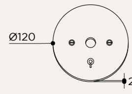
BP02SW universal electrical box with toggle switch
