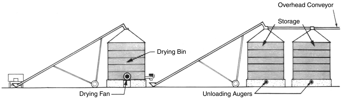
Figure 16. Handling system for a bin dryer using portable augers. Overhead conveyors connect to several storage bins.
