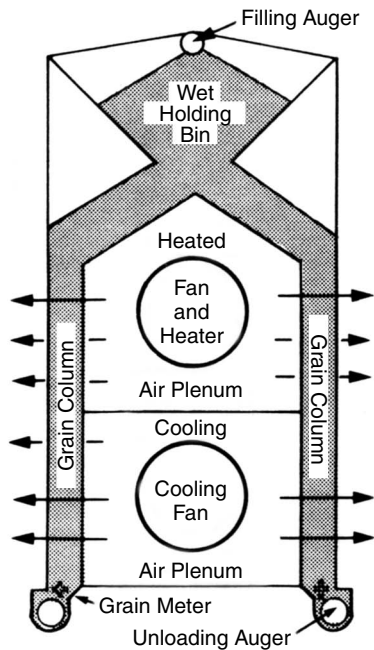
Figure 7. Cross-flow dryer with forced-air drying and cooling.
