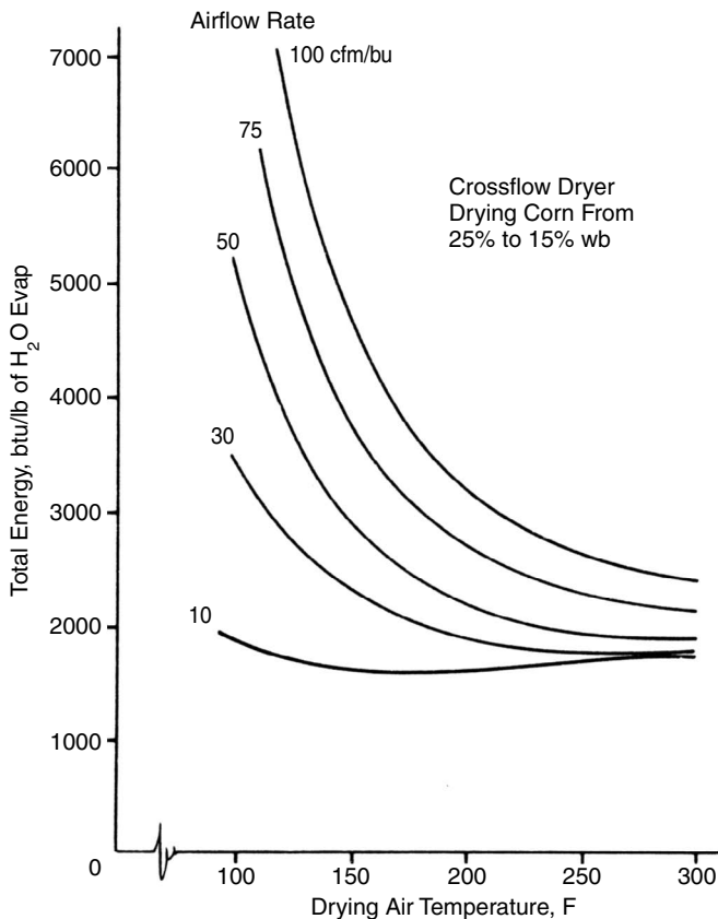
Figure 12. Energy requirements of a conventional crossflow dryer as a function of drying air temperature and airflow rate. (University of Nebraska)
