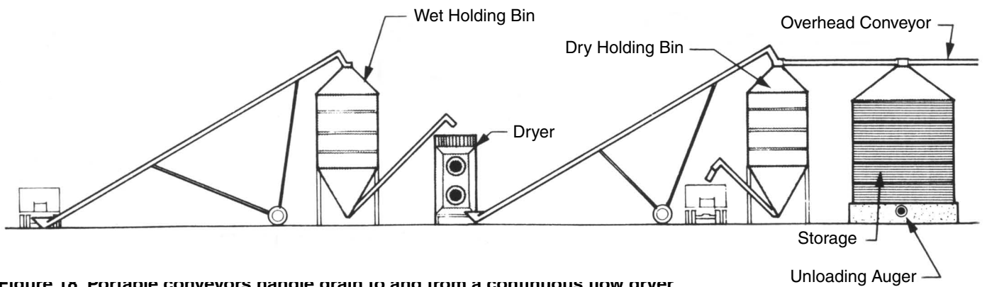
Figure 18. Portable conveyors handle grain to and from a continuous flow dryer.
