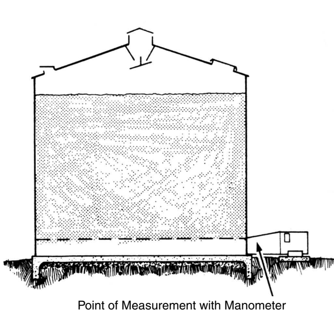
Figure 13. A U-tube manometer used for measuring static pressure.
