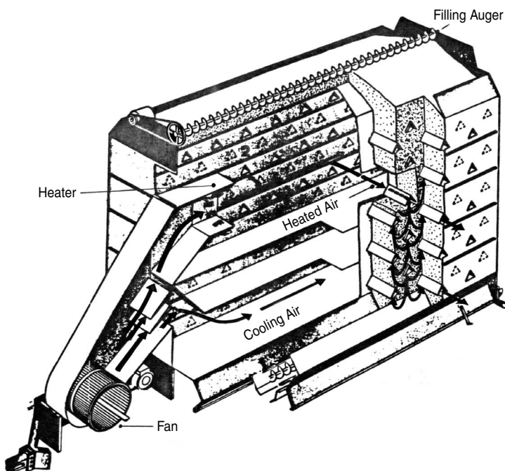
Figure 10. Mixed-flow dryer.
