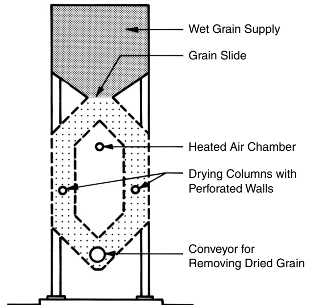
Figure 5. Cross-section of a column batch dryer.
