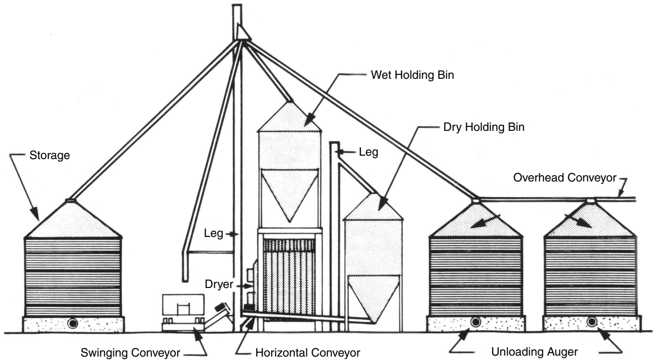
Figure 19. A completely mechanized grain handling-drying system using all permanently installed handling equipment.
