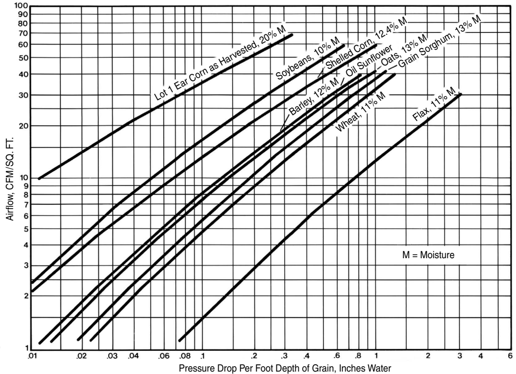
Figure 14. Resistance of clean grains to air flow. Multiply values by 1.3 to 1.5 to adjust for packing and foreign material. Using a grain distributor will increase the resistance to airflow.
