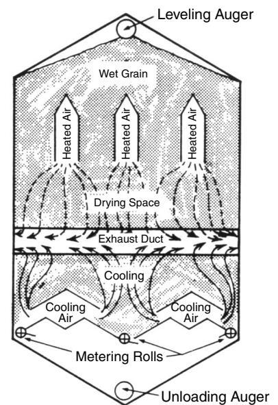
Figure 9. Schematic of a concurrent-flow dryer with counter-flow cooling.
