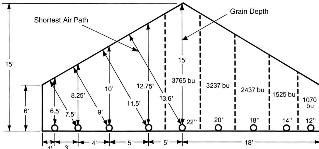
Figure 2. Duct size and spacing for natural air drying in a 36' x 72' building with grain 6 feet deep next to the walls and 15 deep in the center. Perforated duct diameter varies due to different amounts of air required.
