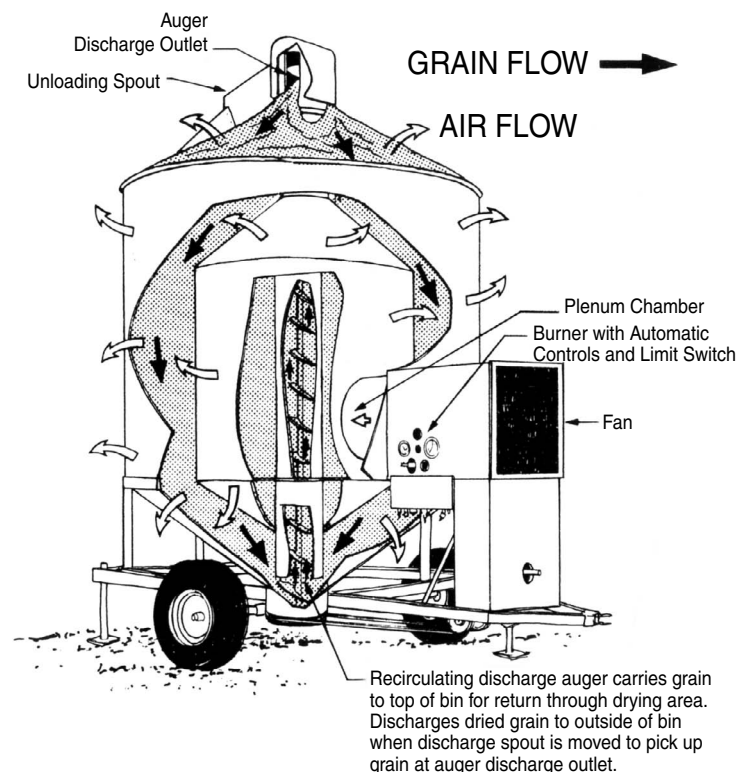
Figure 6. Recirculating batch dryer.
