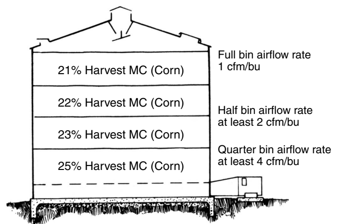
Figure 3. Example of layer drying. The higher airflow rates on a per bushel basis early in the filling permit a higher initial moisture content to be loaded.
