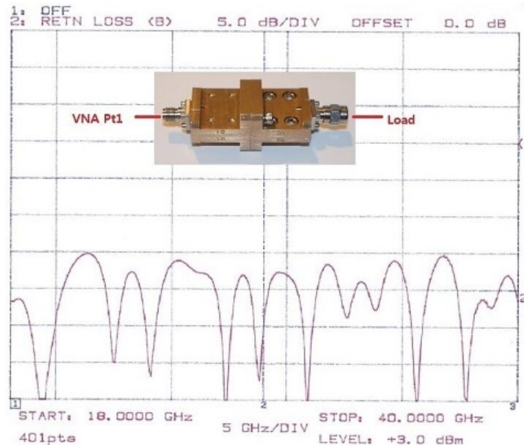
Measured return loss. 15 dB min. over 18.0 - 40.0 GHz in back-to-back configuration
