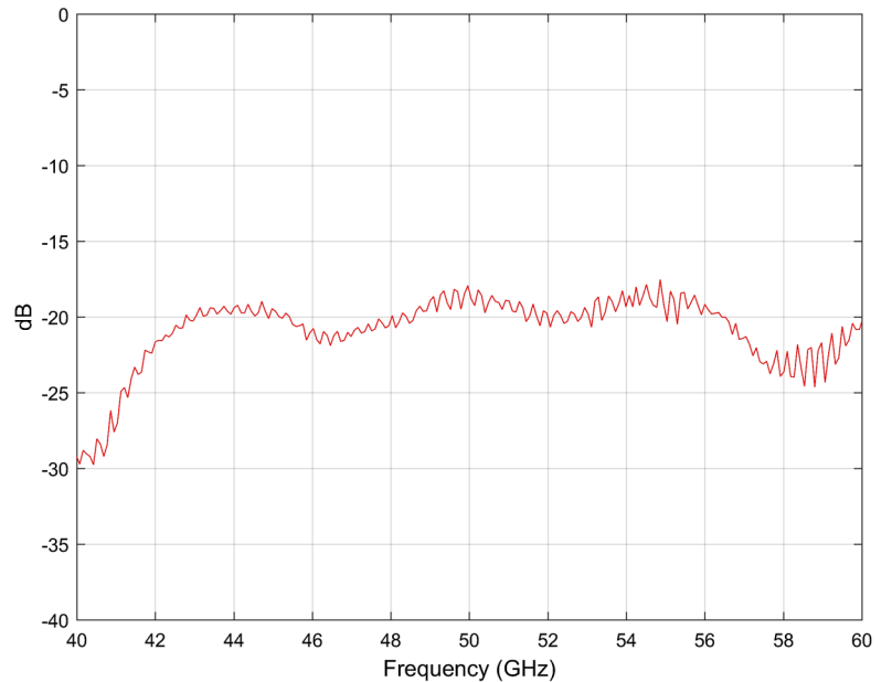
TRCW-198F(M)RC0, Reflection:
