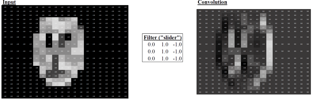
Figure IA.1. Simplified example of convolution. The fictional input image (left) with 20 \times 20 pixels is roughly recognizable as a face. In this fictional image, each pixel (“cell”) is encoded with a number between -1 and +1 determining its color, with -1.0 defined as black and +1.0 defined as white. The output image (right) is obtained through convolution. The 3 \times 3 filter matrix (center) slides over each possible 3 \times 3 region in the input image and outputs the sum of element-wise matrix multiplication of these 3 \times 3 image regions and the filter matrix. Example inspired by material by Jeremy Howard ( youtube.com/watch?v=V2h3IOBDvrA ) and deeplizard ( deeplizard.com/learn/video/YRhxdkVsIs ).
