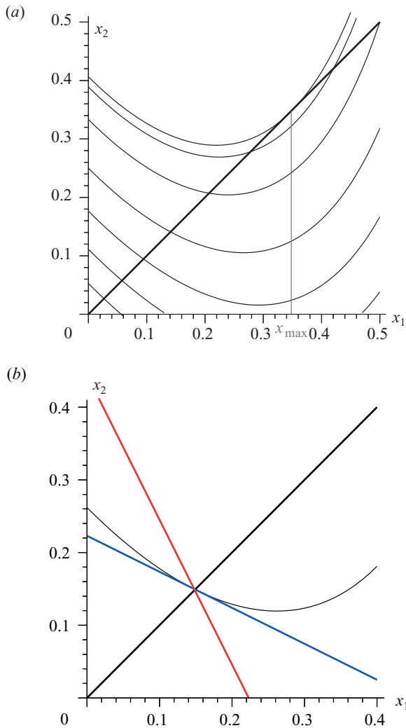
Figure 4. (a) Some level curves of W . At points on the diagonal x_1 = x_2 = x between x = 0 and x = x_{\max} these curves have slope between -1 and 1 . (b) The (x_1, x_2) configuration at the equilibrium point \lambda^* = 0.5 , \rho^* = 0.223 depicted in figure 2. The response lines for players 1 (red) and 2 (blue) both intersect the diagonal at \hat{x}^* = 0.1486 and the level curve for the fitness F(x_1, x_2) is drawn through that point. The response line for player 2 is tangent to that curve, indicating that player 1 cannot increase its fitness by moving its response line (red) to another location. The negotiated contributions are determined at the intersections of the red and blue lines.
