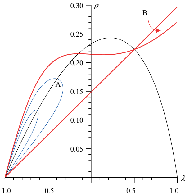
Figure 6. Curves of constant mutant fitness in a population with resident strategy \lambda^* = 0.5 , \rho^* = 0.223 at frequency p = 0.8 and mutant strategy (\lambda, \rho) at frequency p = 0.2 . The level curve \Delta W = 0 (red) consists of the neutral line and a curve that starts at (-1, 0) on the left, rises above the equilibrium curve, and then crosses it twice, the second time at the equilibrium point (\lambda^*, \rho^*) . The region between this curve and the neutral line is the region of positive \Delta W and consists of the two regions marked A and B. The blue contours \Delta W = 0.005 (outer) and \Delta W = 0.01 (inner) are also included.
