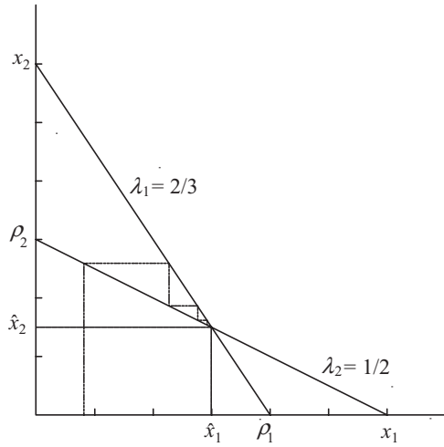
Figure 1. The negotiation process is illustrated for players with linear response rules (player 1, x_1 , has \lambda_1 = 2/3 and \rho_1 = 0.4 and player 2, x_2 , has \lambda_2 = 1/2 and \rho_2 = 0.3 in equation (2.1)). Note that the x_2 -response line uses the x_1 -axis as the abscissa, and it projects any x_1 offer onto the x_2 -axis. Similarly, the x_1 -response line uses the x_2 -axis as the abscissa, and projects any x_2 offer onto the x_1 -axis. In the negotiation illustrated, x_1 begins, and its successive offers are given by successive vertical lines moving from left to right. The responses by x_2 are given by successive horizontal lines moving from top to bottom. The final contributions are at the intersection of the response lines, at \hat{x}_1 = 0.3 and \hat{x}_2 = 0.15 .
