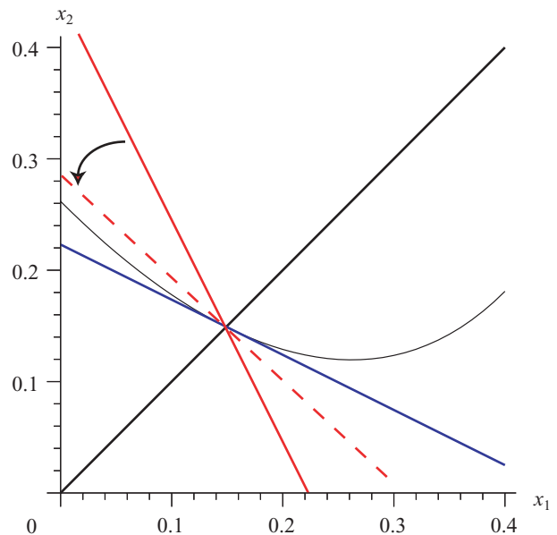
Figure 5. Any response line for player 1 (dashed) which intersects the diagonal at \hat{x}^* will have resident fitness. These are the response lines that correspond to the neutral line in figure 2.
