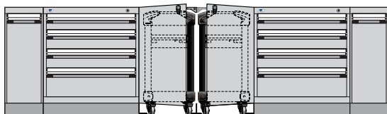
2 Toolboxes - 2 Hideaway Doors - 2 Lift Control Units 2 MultiTek Carts
