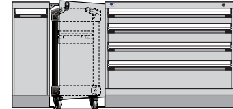
Toolbox - Hideaway Door - Lift Control Unit MultiTek Cart GT-B072B02AR4C2_
