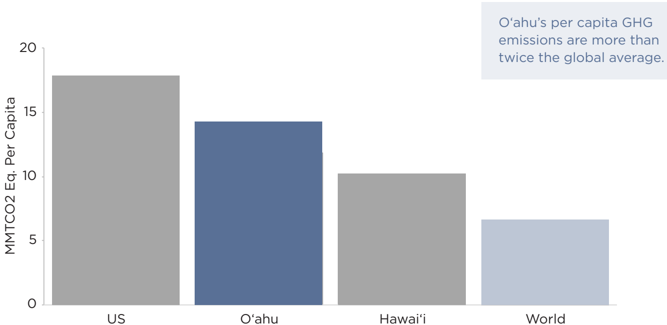
Figure 3: Comparison of 2016 Per Capita GHG Emissions
