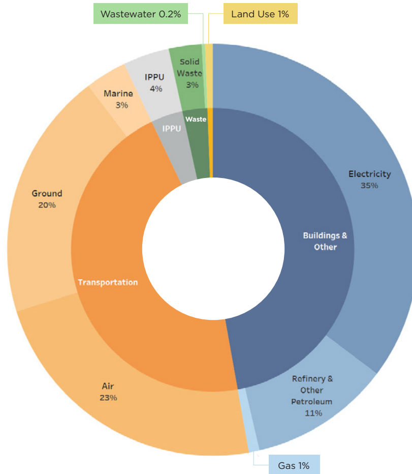
Figure 2: O‘ahu’s GHG Emissions by Detailed Sector, 2017
