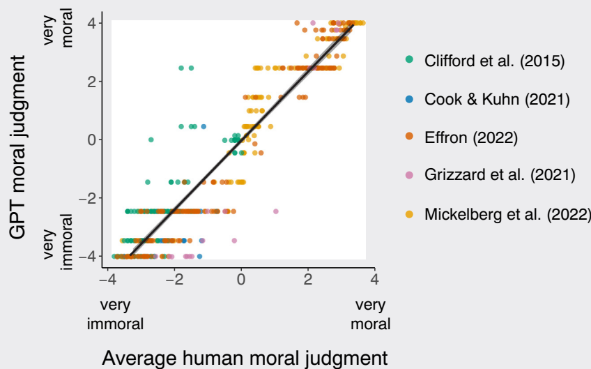
Figure 1. Comparing the moral judgments of humans versus GPT. Refs used in figure [5–9]
