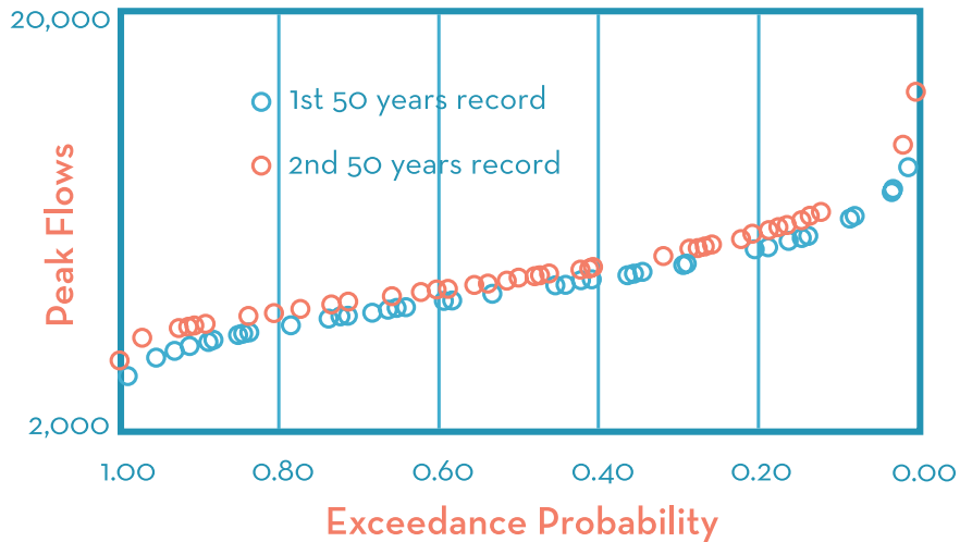
Figure 2.7. A log Pearson III fitting of one hundred years of maximum annual peak flows (in m^3/s ) in the Waas River Basin. A fitting was made for the first and second 50 years of observed data.
