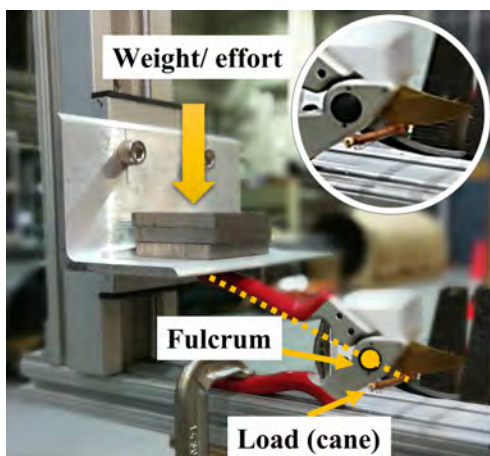
Figure 5: Experimental setup to measure force required to cut dormant canes (left) with a bypass pruner. Correlation plot between cane diameter and cutting force (right).
