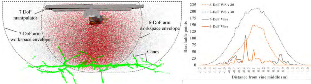
Figure 18: Top view of the work volume of the 6 and 7 DoF arms (left) separated by the dashed line. The red and black dots are reachable positions for the 6&7 DoF respectively. A graphical representation of the reachable locations in the vine for both 6 and 7 DoF arm (right).
