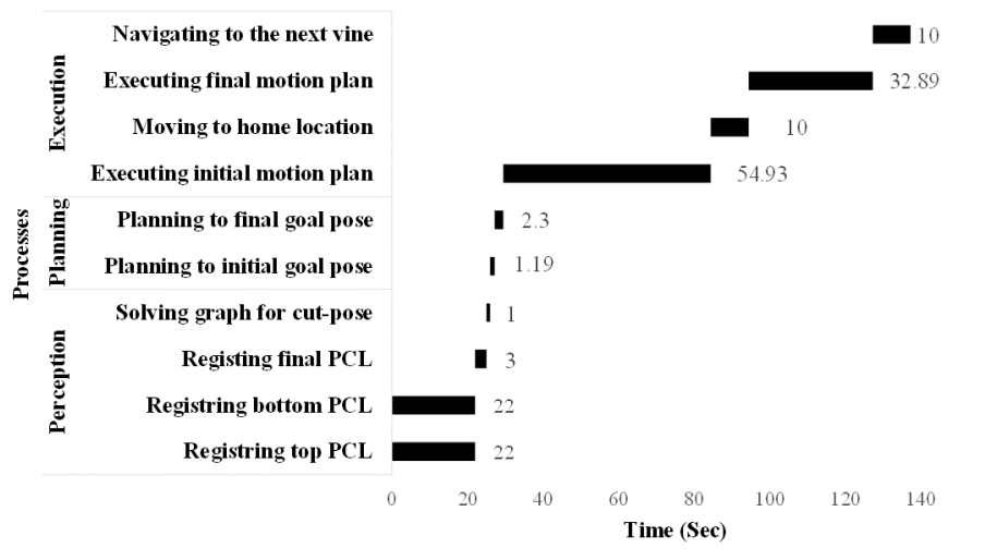
Figure 19: Total computation time breakdown for pruning a vine from a single side of the canopy.
