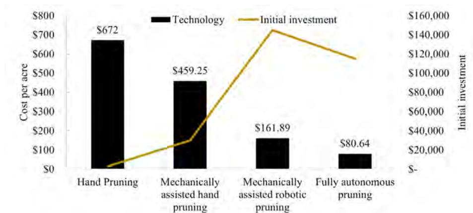
Figure 23: Cost breakdown for different pruning technologies.
