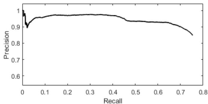
Figure 16: The P-R curve for bud detection network with Faster-RCNN network (left). Each yellow bounding box localizes a bud in the image (right).
