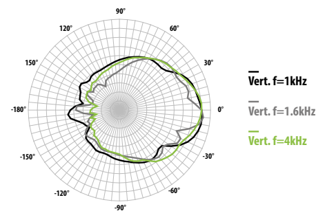
Ver. Polarplots, 6 dB/div
