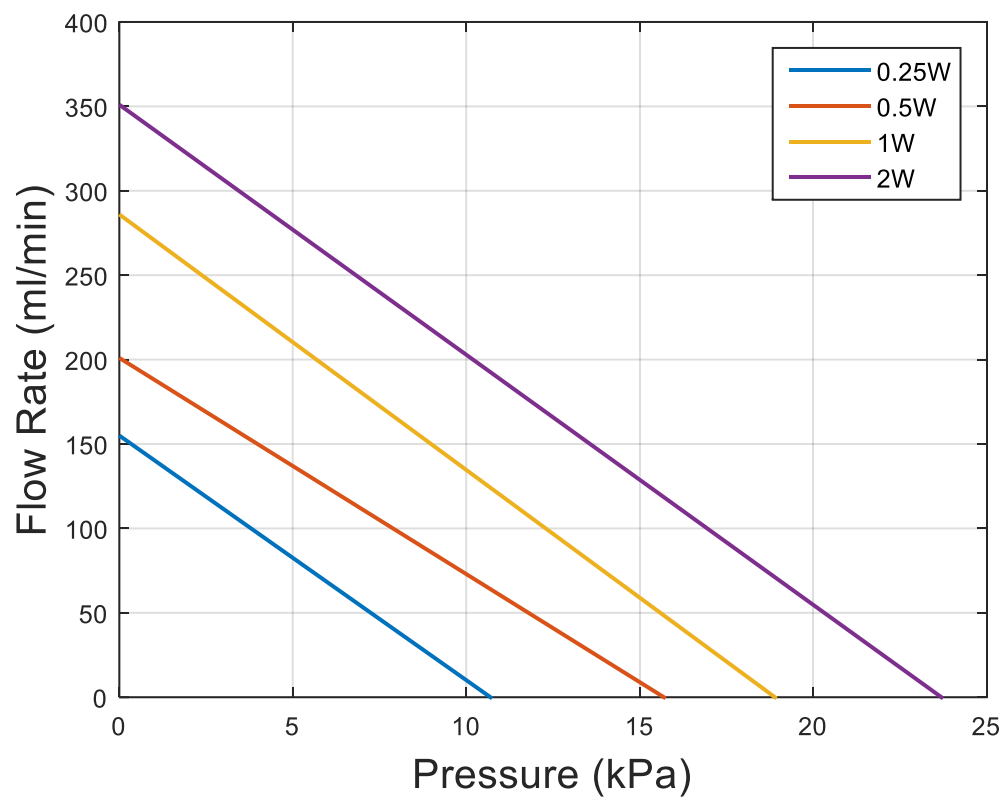
Pressure Flow-rate characteristics at 0.25, 0.5, 1, & 2 W
