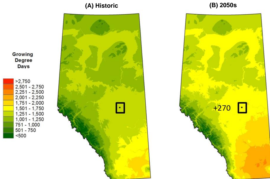
Figure 6: (A) Historic (1961-1990) and (B) projected distribution of growing degree days in Alberta by the 2050s (2041-2070) xiii
