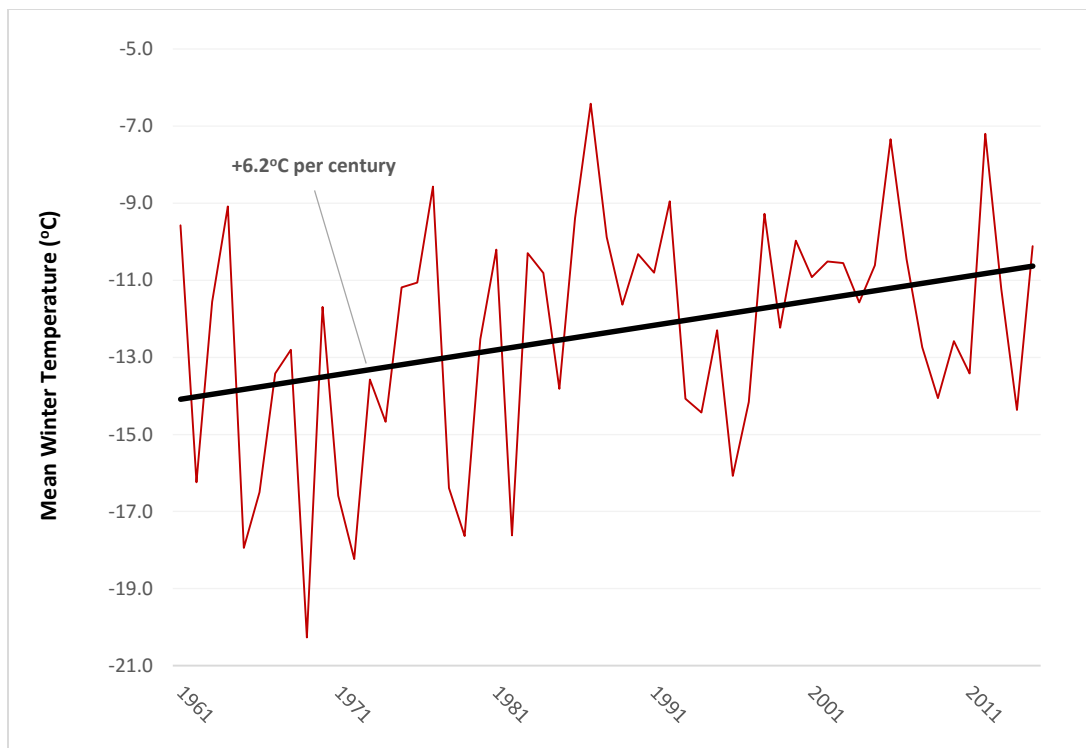
Figure 3: Mean winter temperature in the Bruderheim area (1961-2015)
