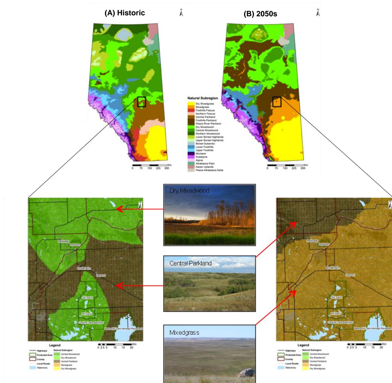
Figure 7: (A) Historic (1961-1990) and (B) projected (2050s) distribution of natural sub-regions in Alberta and in the Bruderheim area xviii,xix
