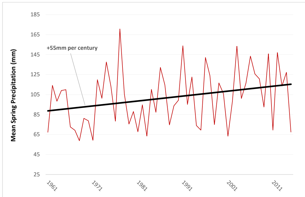
Figure 4: Mean spring precipitation in the Bruderheim area (1961-2015)
