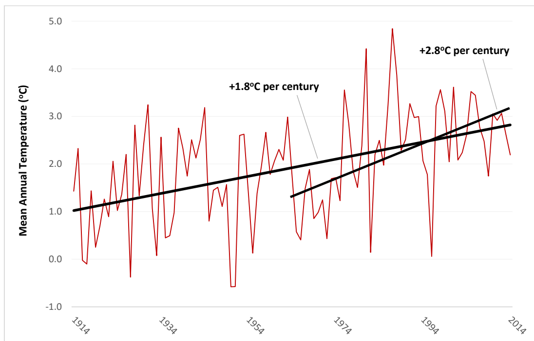
Figure 2: Mean annual temperature in the Bruderheim area (1914-2014)
