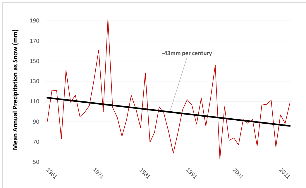
Figure 5: Precipitation falling as snow in the Bruderheim area (Sept-Jun) (1961-2013)
