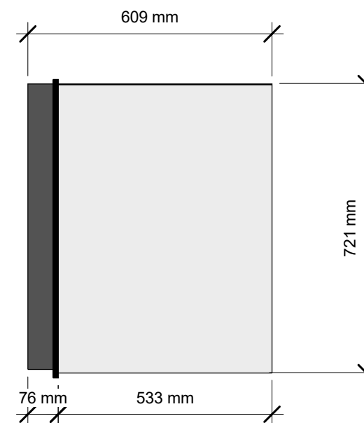
④ SIDE VIEW 1 : 12
