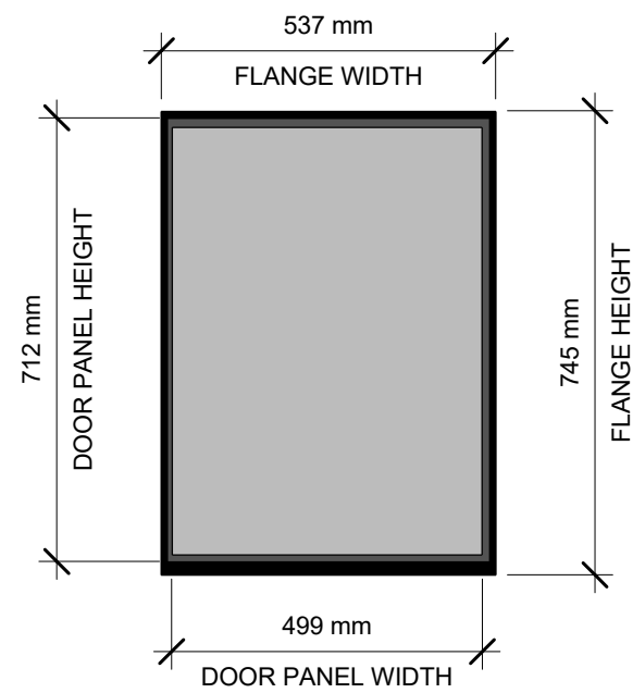
③ FRONT VIEW 1 : 12
