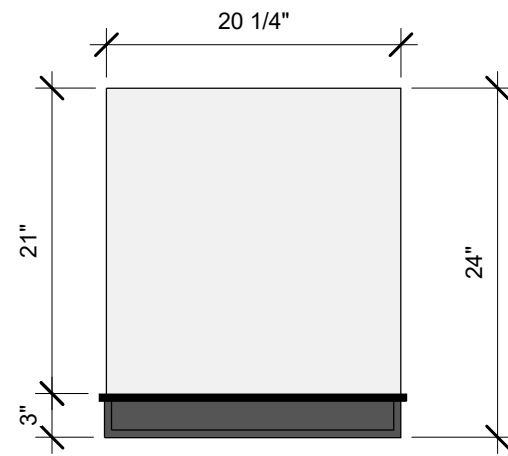
① TOP VIEW 1" = 1'-0"
