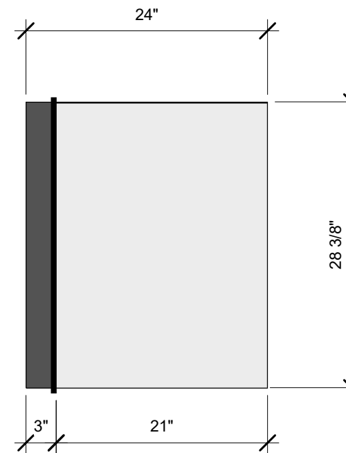
④ SIDE VIEW 1" = 1'-0"
