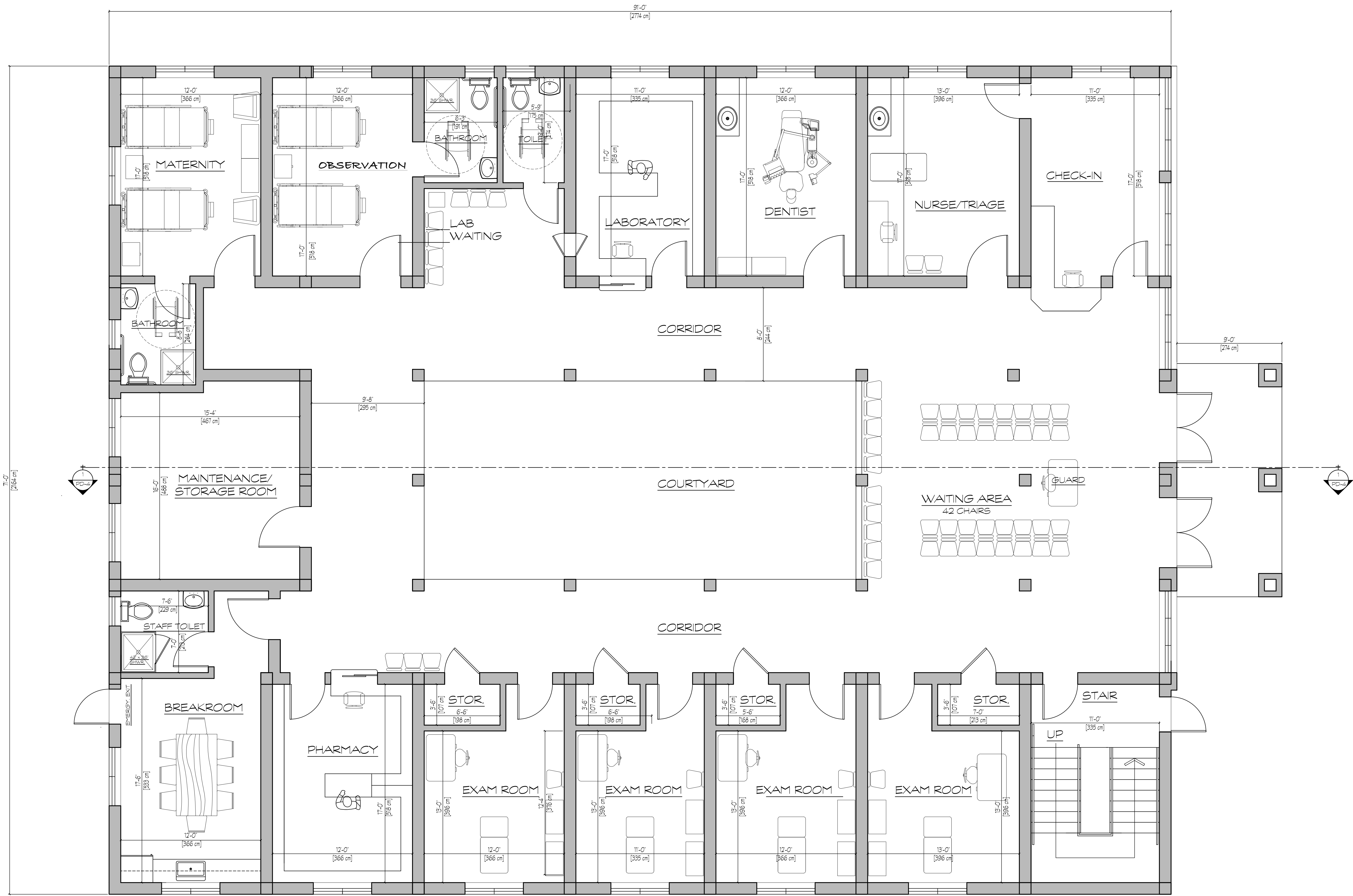
GROUND FLOOR PLAN - 5,832 S.F. [542 Sq. M] SCALE: 1/4" = 1'-0"
