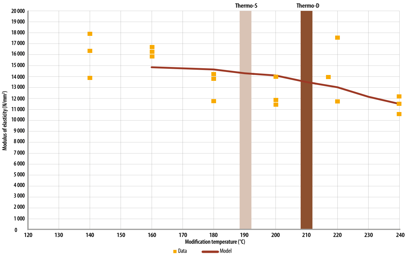
Figure 24. The impact of the modification temperature on the modulus of elasticity of ThermoWood® (source: VTT).
