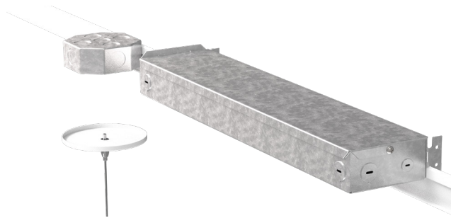
Grid-mountable driver housing with integrated T-Wing mounts.
