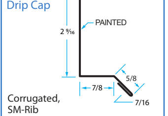
DC-1 Drip Cap
