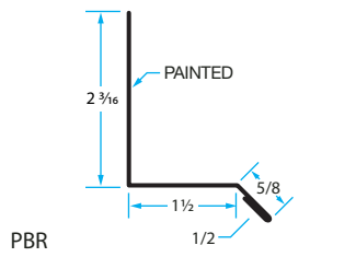
DC-2 Drip Cap
