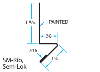
BD-1 Base Drip
