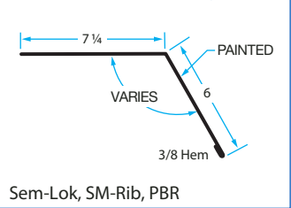
GF-1 Gambrel Flashing
