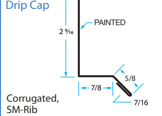
DC-1 Drip Cap
