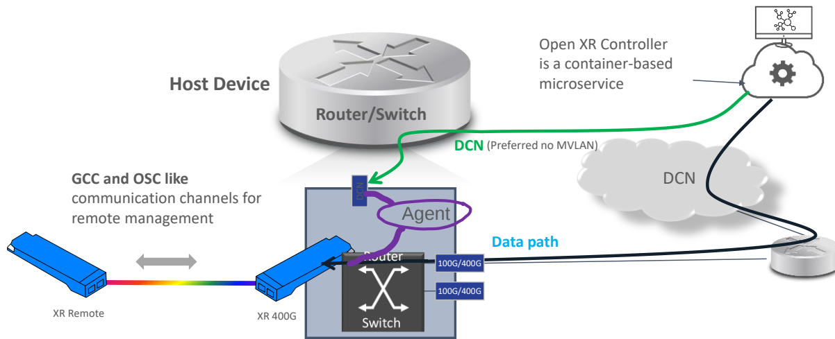
Figure 5. Open XR module management via data path
