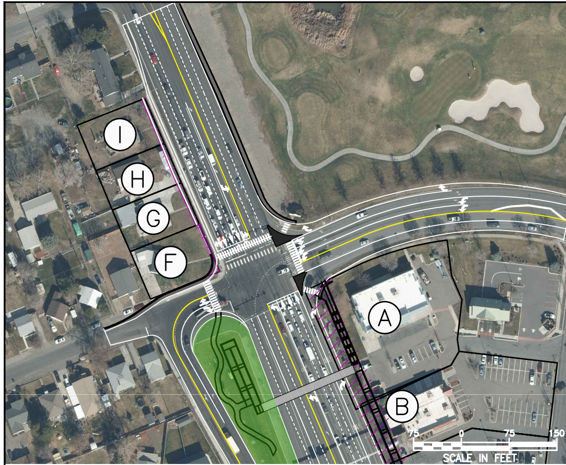
INTERSECTION DETAIL
