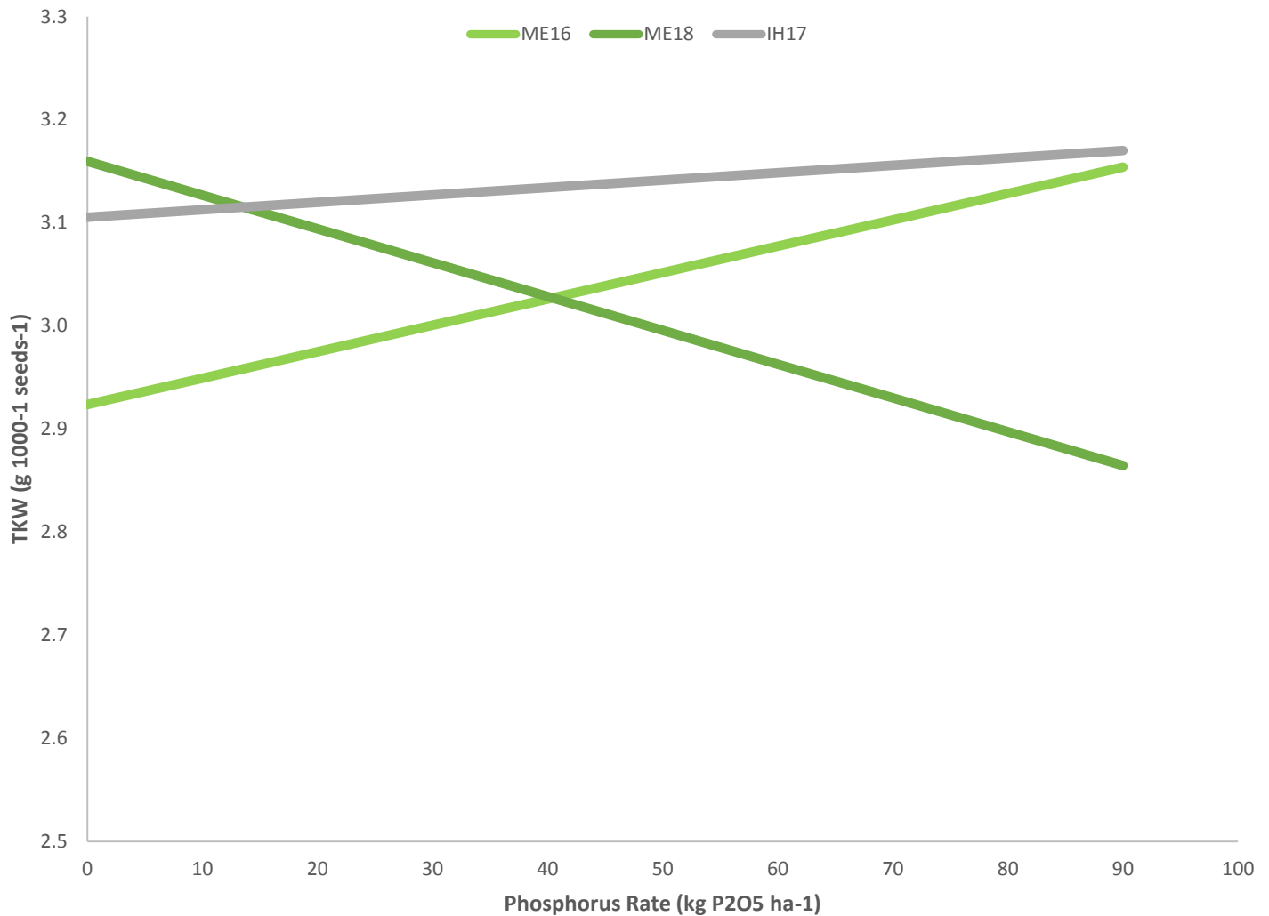
Figure 29. Phosphorus Rate (kg P 2 O 5 ha -1 ) Effect on Thousand Kernel Weight (g 1000 -1 seeds -1 ) at Three Site-years.
