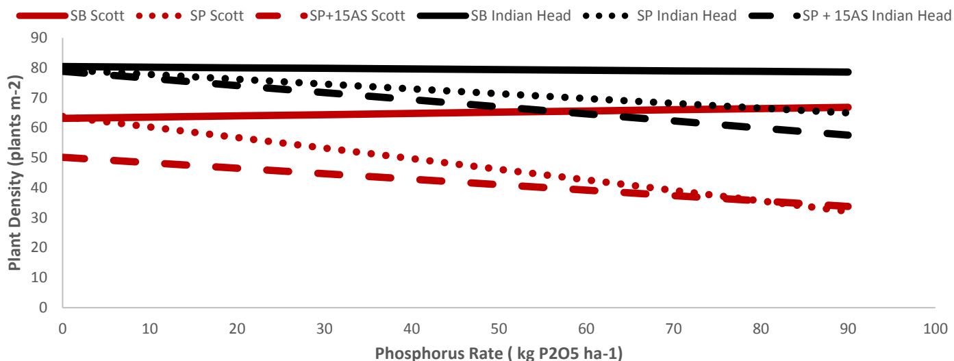
Figure 9. Phosphorus Rate and Placement Interaction Effect on Plant Density (plants m -2 ) Four Weeks after Seeding at Scott and Indian Head, Combined over Three Years.
