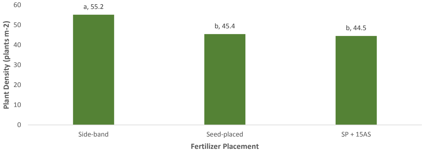
Figure 14. Phosphorus Placement Effect on Plant Density (plants m -2 ) Six Weeks after Seeding at Melfort Combined over Three Years.
