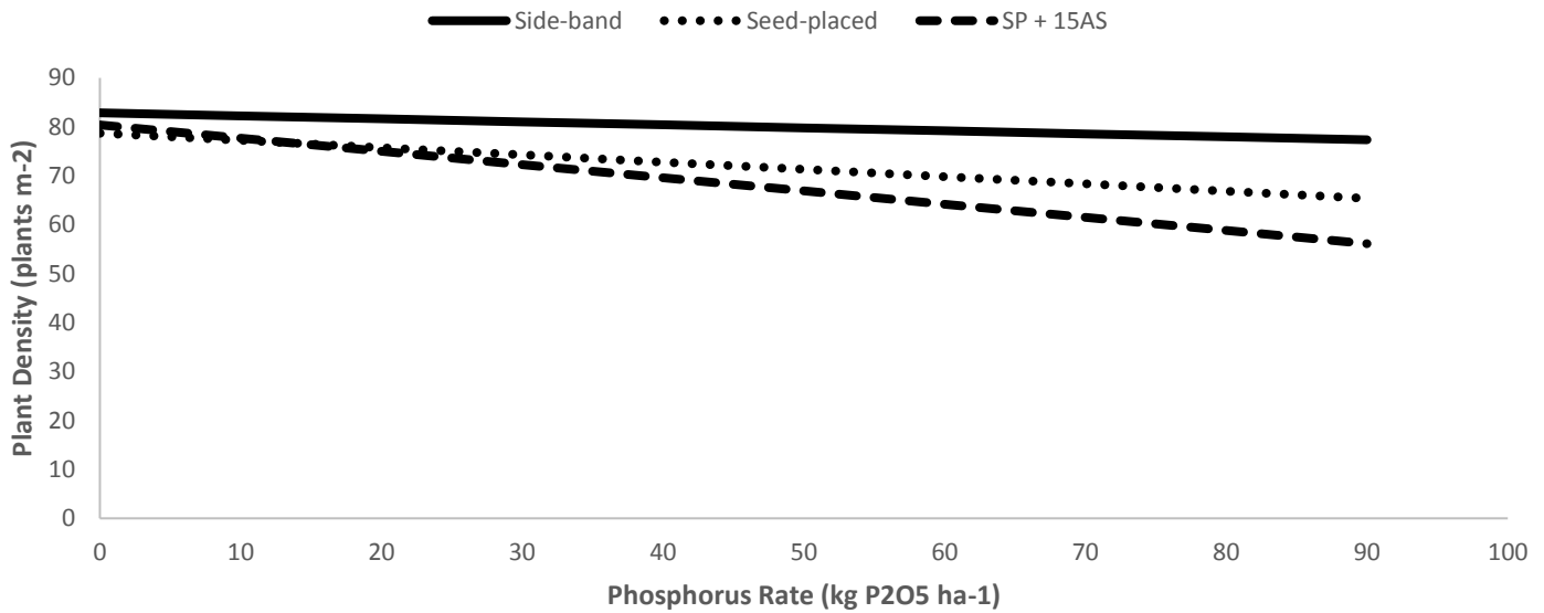
Figure 15. Phosphorus Rate (kg P 2 O 5 ha -1 ) Effect on Plant Density (plants m -2 ) Six Weeks after Seeding at Indian Head Combined over Three Years.
