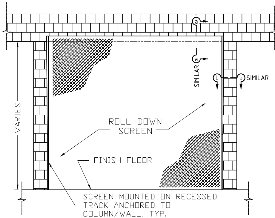
ELEVATION VIEW
