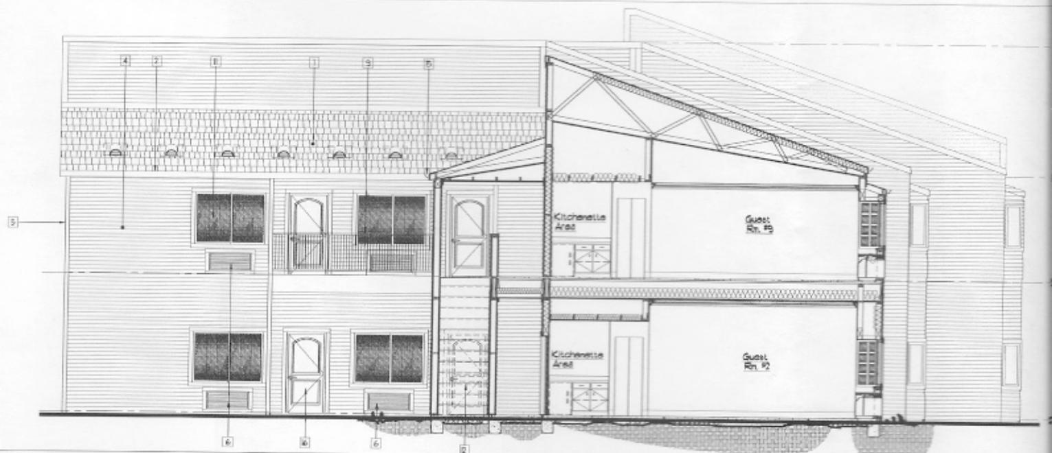
East Elevation
