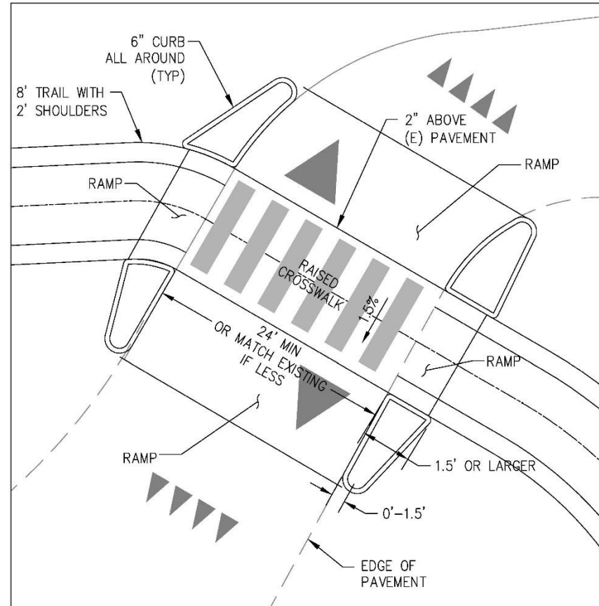
RAISED CROSSING
