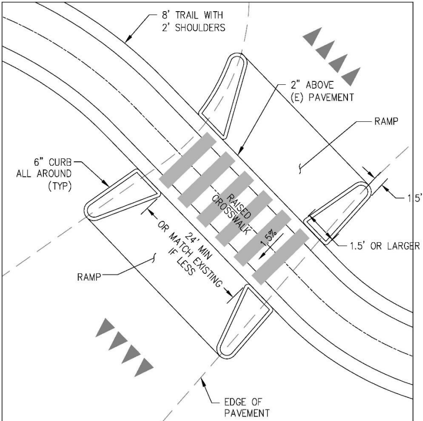
RAISED CROSSING (CHOKER)
