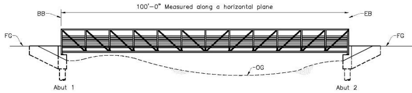
ELEVATION 1"=10'-0"
