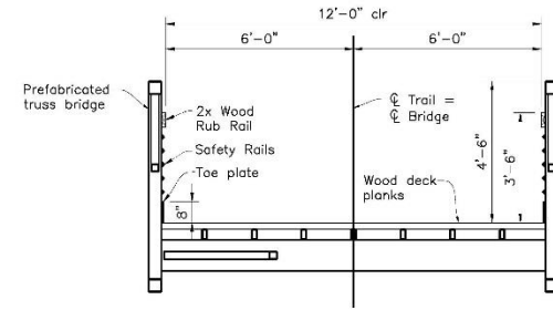
TYPICAL SECTION 1/2"=1'-0"
