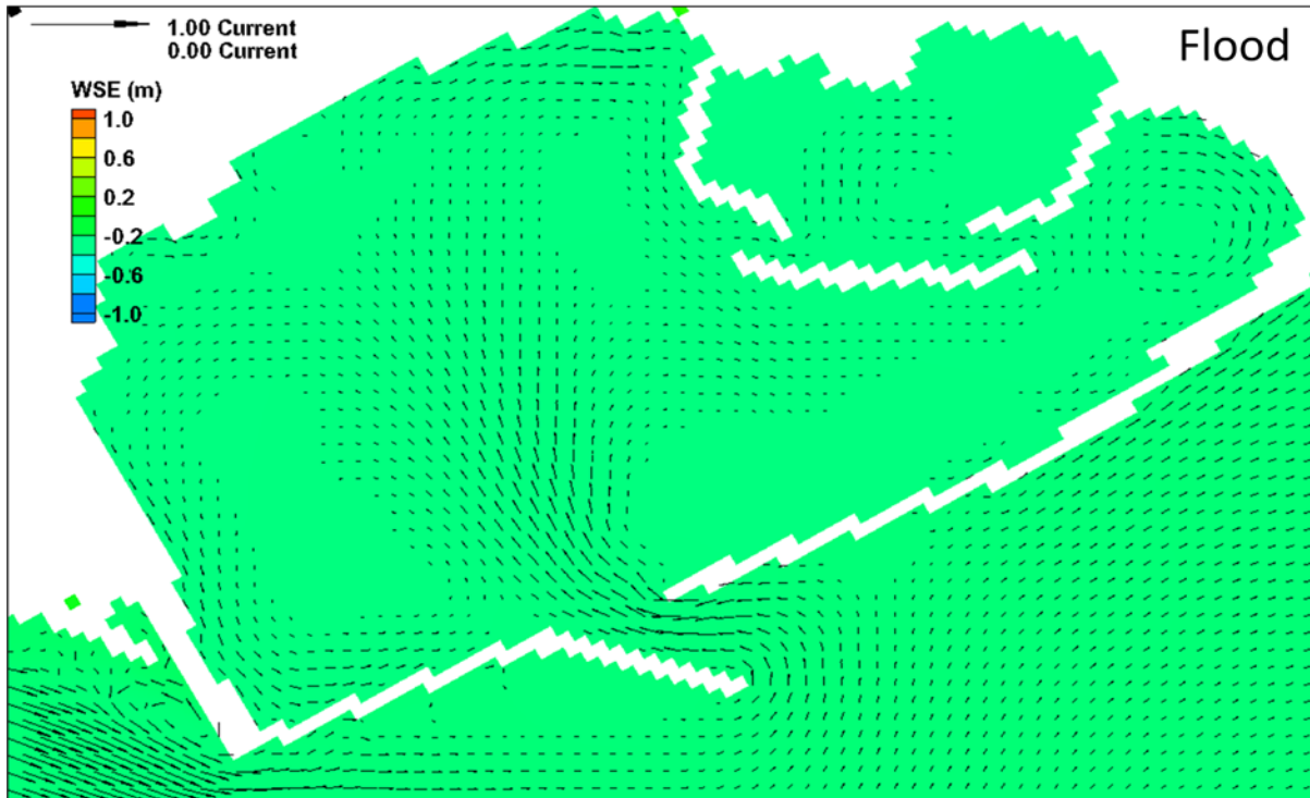
Figure 37. Circulation in Half Moon Bay during the flood tide
