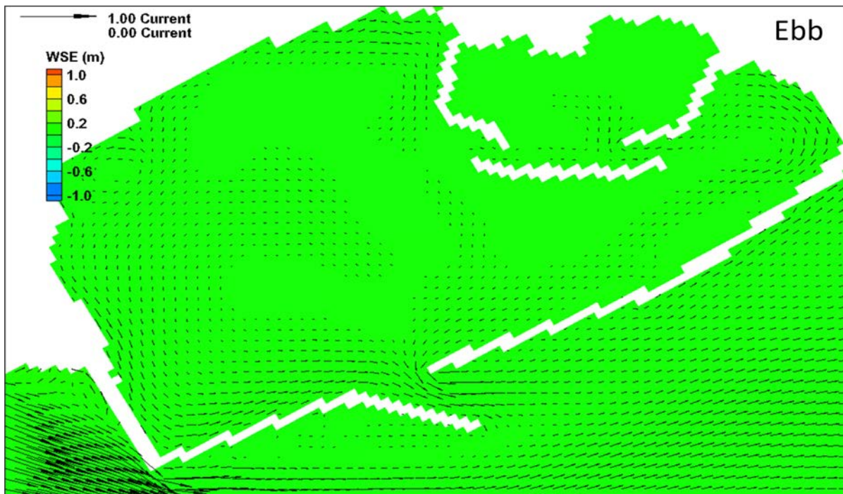
Figure 38. Circulation in Half Moon Bay during the ebb tide
