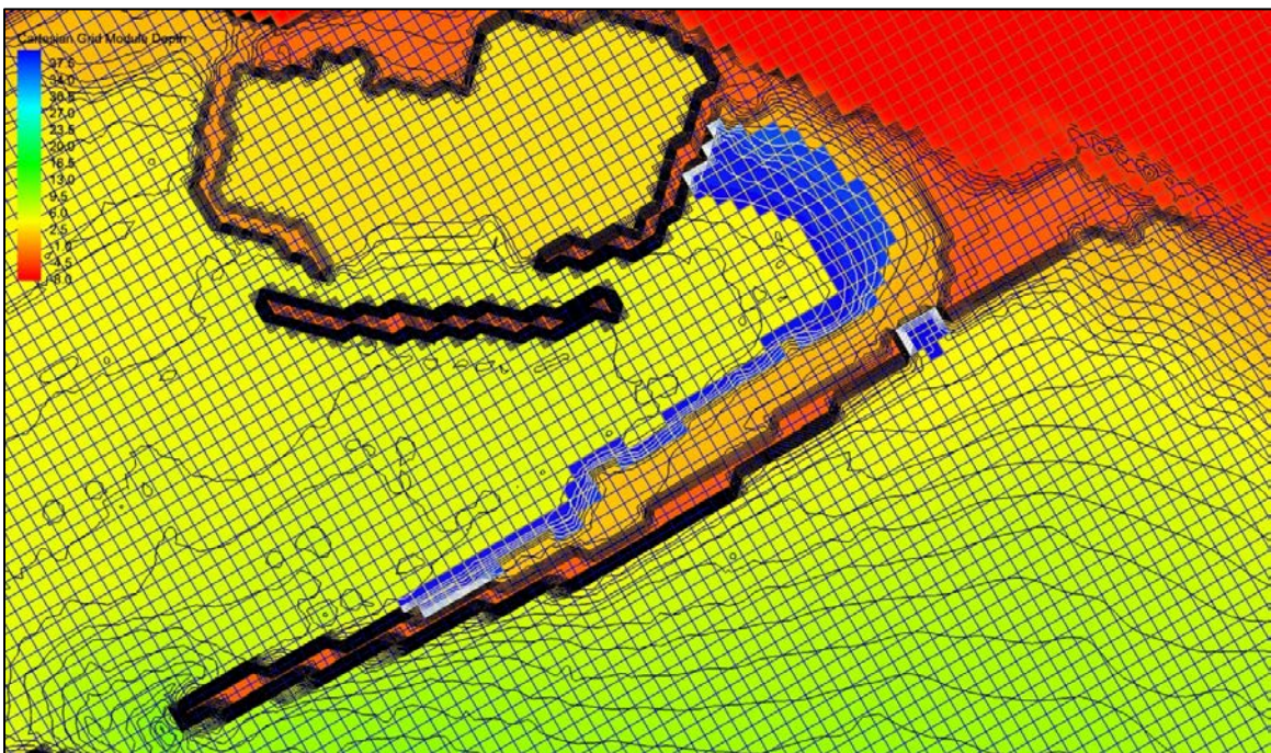
Figure 65. Cells specified as “limited erodible cells” with a limit of 0.6 m, as it was assumed that sand in these areas was at least 0.6 m (2 ft) deep
