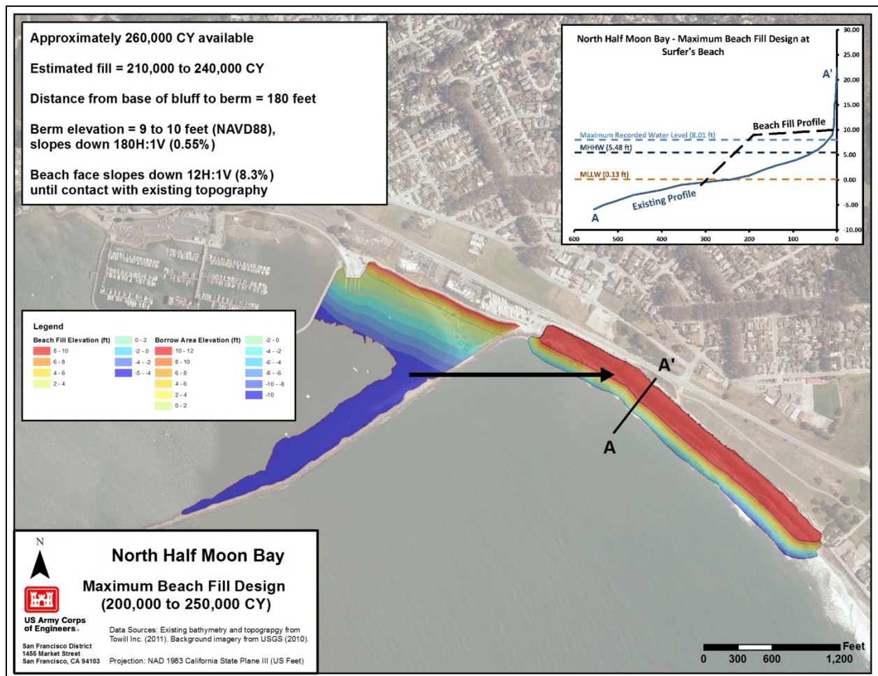
Figure 54. Schematic of maximum beach fill design scenario
