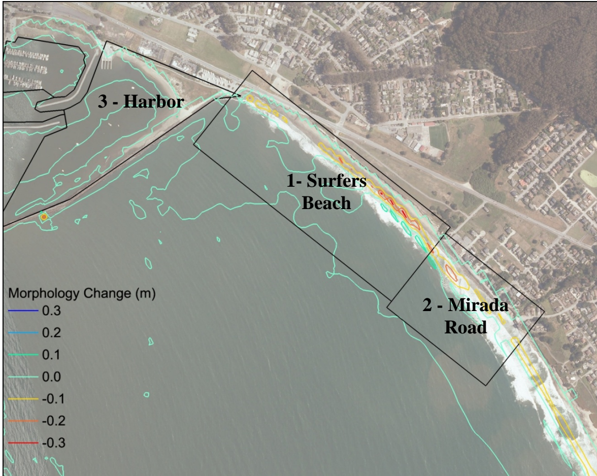
Figure 44. Calculated morphology change in the vicinity of Surfers Beach from June 2009 to November 2009 (6 months). The boxes (1 – 3) outline the analysis areas
