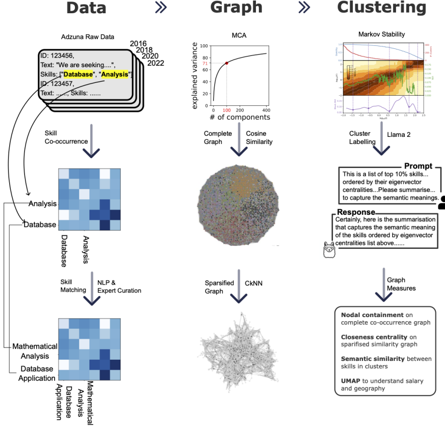
Figure 1: From job postings to the clustering of a network of co-occurrent skills: (a) the data preparation including the extraction of skill co-occurrence from metadata, skill matching to Lightcast taxonomy and dimensionality reduction using MCA; (b) the graph-based clustering including the sparsification of the complete cosine similarity graph and the multiscale clustering with Markov Stability; and (c) the descriptive analysis on the optimal clustering with 21 partitions using LLM, nodal containment and closeness centrality.
