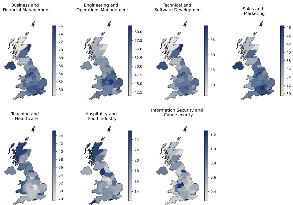
Figure 17: Maps for each of the MS7 clusters showing the percentage of all adverts in each NUTS2 regions featuring a skill from the cluster.
