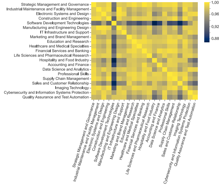
Figure 7: Coverage between MS21 clusters. Coverage of the coarse-grained co-occurrence matrix K obtained by: (i) computing B = U^T K U where U is the matrix where U_{ij} that records the number of mentions of a skill i in cluster j ; (ii) normalising B_{ij} by \sqrt{B_{ii} B_{jj}} . Coverage and containment have opposite meanings: the ‘Software Development Technologies’ cluster has high self-containment (i.e., low values of its coverage), and is especially unlikely to co-occur with ‘Sales and Customer Relationship’ or ‘Hospitality and Food Industry’.
