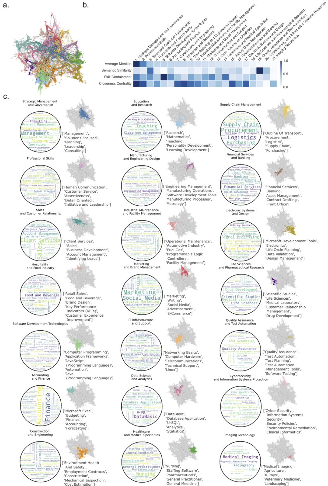
Figure 5: Co-occurrence skill clusters (MS21) (a) Skills network coloured according to the 21 skill clusters. (b) Summary heatmap of skill clusters properties. Each row is normalised by its maximum. (c) For each of the 21 clusters, word cloud where font size represents skill eigenvector centrality, and list of top 5 most frequent skills.
