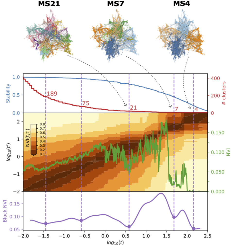
Figure 2: Optimal clusterings from Markov Stability on the sparsified graph \mathcal{G} . Five optimal highly robust partitions are identified based on minima of the Block NVI. For further details, see text, Refs. [43, 45–47], and Appendix B.
