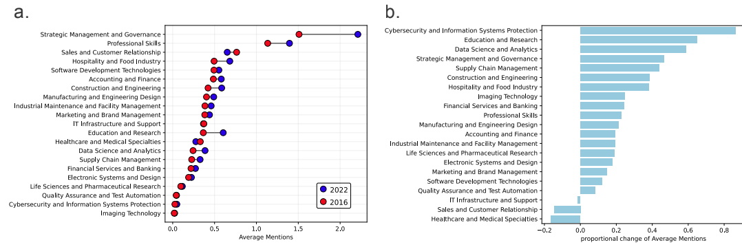
Figure 11: Temporal changes of skill demand. (a) Temporal changes in average mentions for all skill clusters from 2016 to 2022 and (b) the corresponding relative changes.
