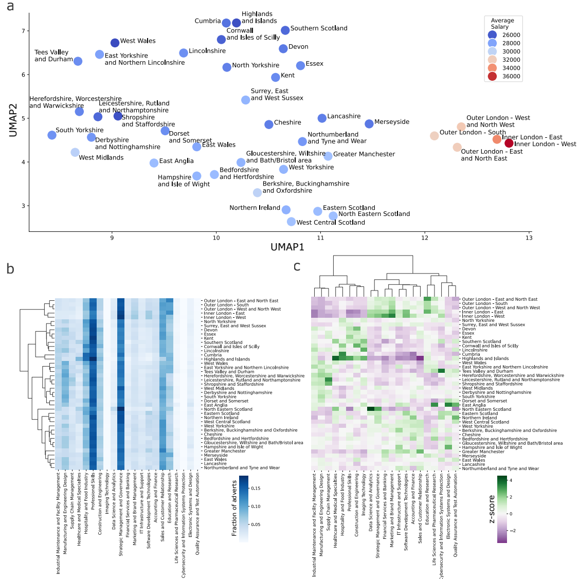
Figure 10: Projection of the skill profiles of NUTS2 regions. (a) UMAP projection of the set of 21-dimensional vectors of percentages in the MS21 skill clusters for all NUTS2 regions. NUTS2 regions with similar skill profiles lie close in this projection. The dots of the NUTS2 regions are then coloured a posteriori according to average salary in the region. (b) Hierarchical clustering of the NUTS2 regions based on their MS21 percentages. (c) Hierarchical clustering of the MS21 clusters based on z-scores across regions.
