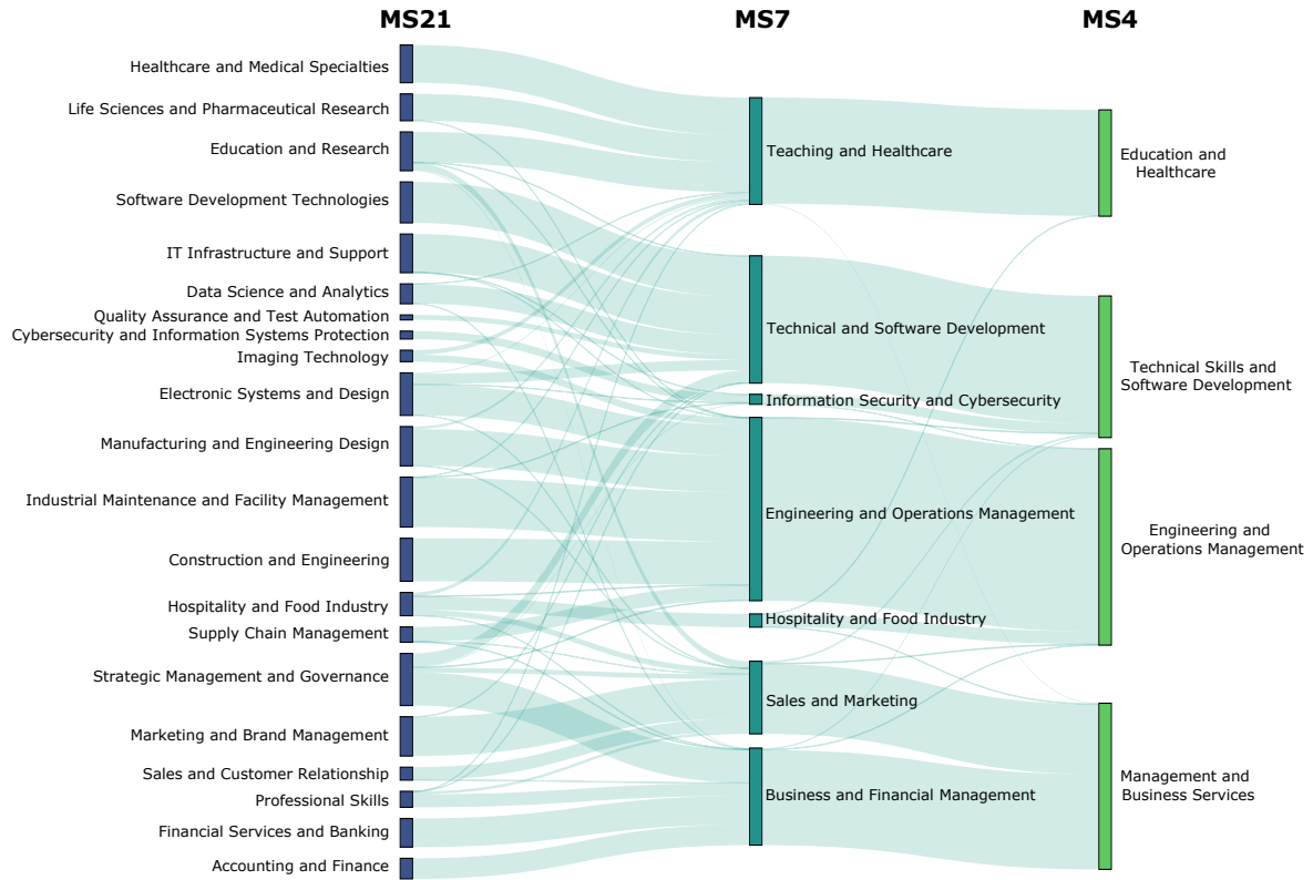
Figure 3: Sankey diagram capturing the multiscale clustering of skills at different levels of resolution. The quasi-hierarchical structure of skill co-occurrences is not imposed by the method but emerges naturally from the intrinsic co-occurrence patterns in the data.
