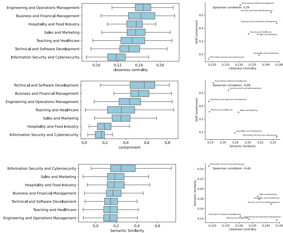
Figure 16: Boxplots for distributions of closeness centrality, skill containment and within cluster semantic similarity for each MS7 skill cluster. The scatter plots compare these three variables.
