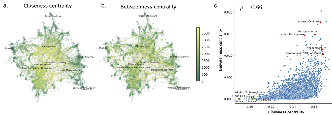
Figure 4: Centrality in the skills network. Skills network with nodes colored by (a) closeness centrality rank and (b) betweenness centrality rank. Yellow indicates high centrality rank, while green indicates low centrality rank. (c) The scatter plot between both centralities shows moderate correlation between them. Some highly mentioned skills with high (red dots) and low (green dots) centrality are indicated.
