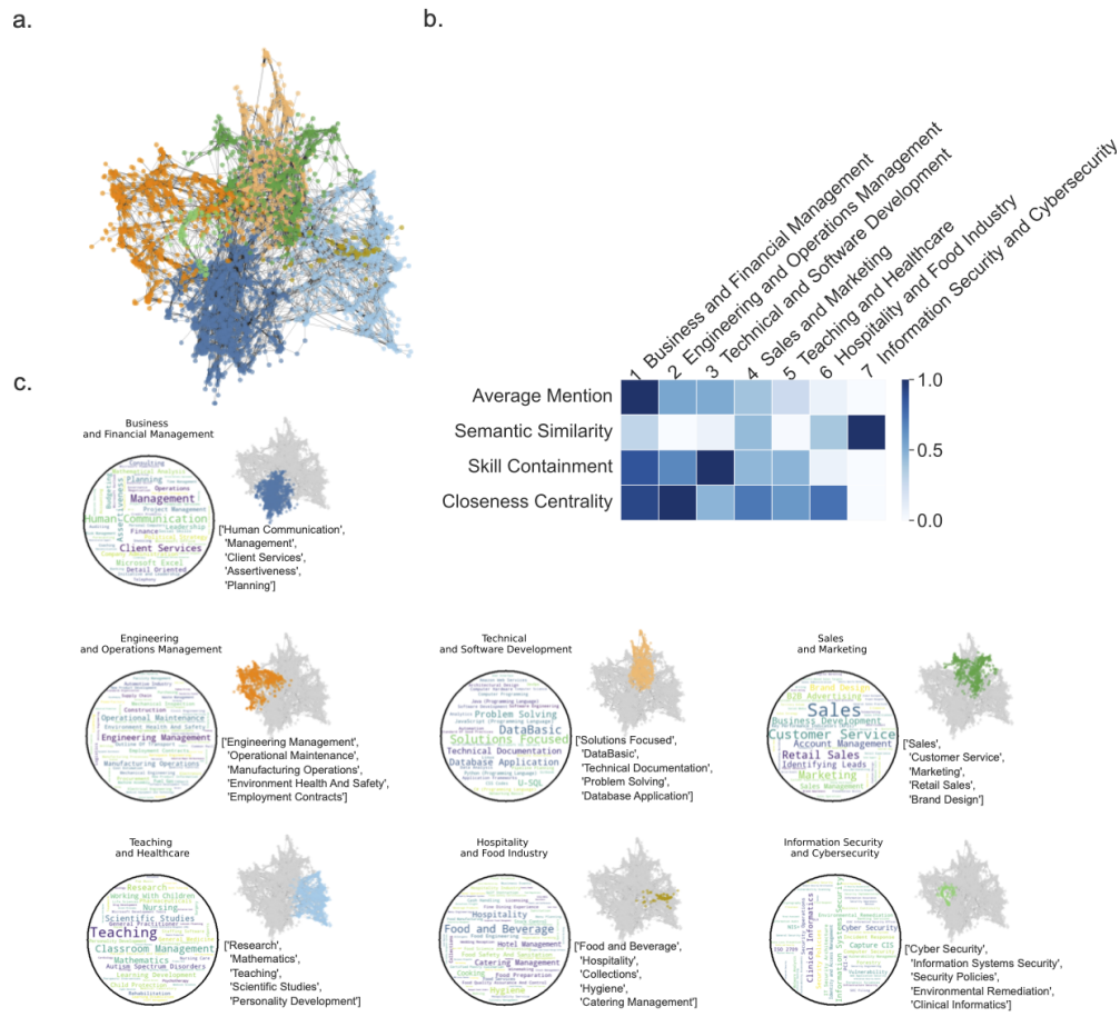
Figure 15: Co-occurrence skill clusters (MS7) (a) Skills network coloured according to the 7 skill clusters. (b) Summary heatmap of skill clusters properties. (c) For each of the 7 clusters, word cloud where font size represents skill eigenvector centrality, and list of top 5 most frequent skills.
