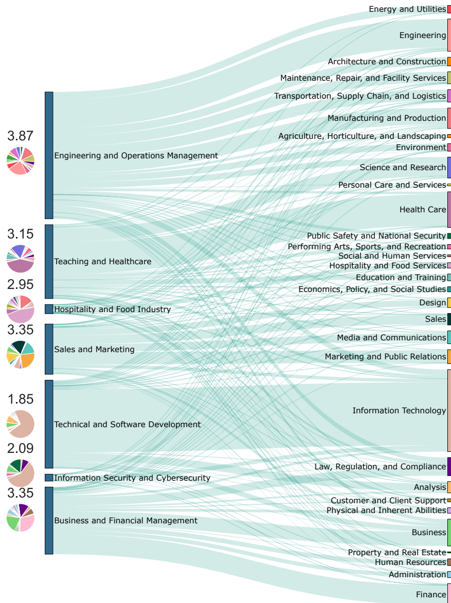
Figure 18: Sankey diagram between co-occurrence skill clusters (MS7) and expert-based skill clusters (Lightcast). There is broad agreement between the data-driven clusters and the LC categories in some skill areas where thematic content and co-occurrence match. For each cluster in MS7, we plot a pie chart to visualise the proportions of Lightcast categories, and the corresponding entropy to indicate how thematically mixed the cluster is.
