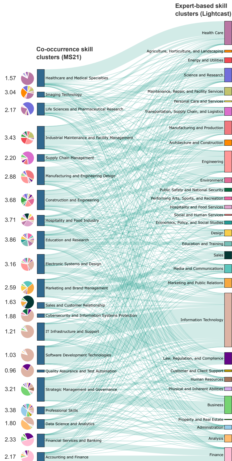
Figure 13: Sankey diagram between co-occurrence skill clusters (MS21) and expert-based skill categories (Lightcast). There is some agreement between the data-driven clusters and the LC categories in skill areas where thematic content and co-occurrence match. For each cluster in MS21, we plot a pie chart to visualise the proportions of Lightcast categories, and the corresponding ‘thematic entropy’ for the skill cluster, which indicates how thematically mixed the cluster 27 .
