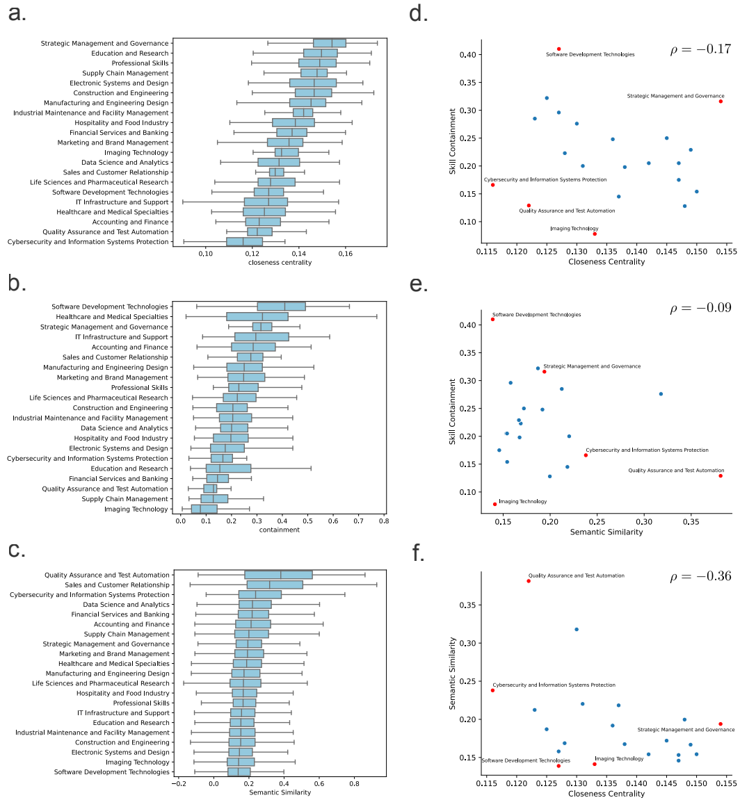
Figure 6: Boxplots for the distributions of (a) closeness centrality (b) containment and (c) within cluster semantic similarity for each cluster. The scatter plots compare for each cluster: (d) median closeness centrality and containment, (e) semantic similarity and containment, and (f) semantic similarity and closeness centrality.
