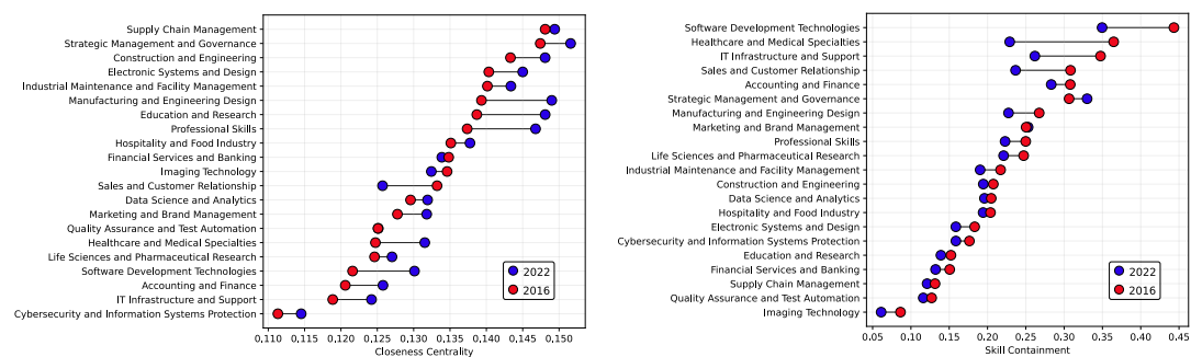
Figure 12: Temporal changes of skill centrality and containment. (a) Temporal change in closeness centrality and (b) skill containment from 2016 to 2022 for all skill clusters.
