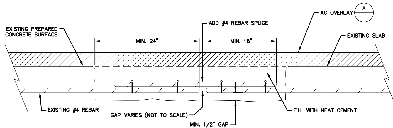
C REPAIR OF DAMAGED REBAR NTS
