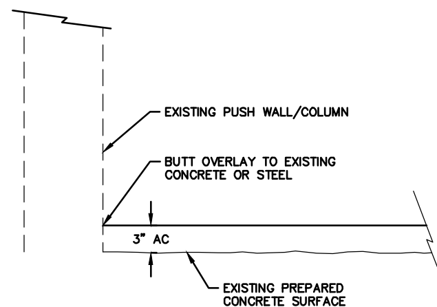
D PUSH WALL/COLUMN TRANSITION NTS
