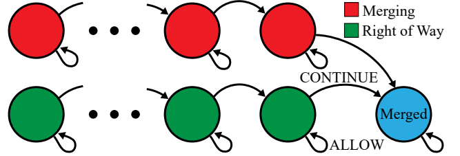
Figure 2: A simplified diagram of the lane merging MDP.
