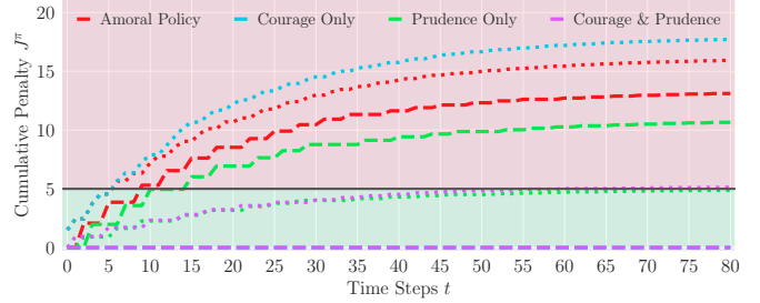
Fig. 4. The cumulative penalty functions for each version of AVE as a function of time steps. Here, the dashed lines denote the cumulative penalty for the courage trait and the dotted lines denote the cumulative penalty for the prudence trait. The solid line denotes a tolerance \tau of 5 and separates the moral region (shaded green ) and the immoral region (shaded red ).
