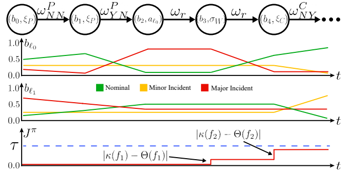
Fig. 1. A campus patrol robot monitors different security feeds and resolves incidents across locations \ell_0 and \ell_1 . Top : The trajectory of the POMDP with belief-action pairs (b, a) connected by observations \omega . Here, the action \xi_P monitors MAJOR incidents with a police scanner, \xi_C monitors MINOR incidents with a camera system, a_\ell navigates to the location \ell , and \sigma_W resolves an incident by warning campus security. Each observation \omega is given by a security feed ( P or C ) and an incident status for the locations \ell_0 and \ell_1 ( Y indicates an incident and N indicates no incident). \omega_r indicates a destination has been reached. Center : The agent’s belief b_f for MINOR and MAJOR incidents at locations \ell_0 and \ell_1 . Bottom : The cumulative penalty J^\pi of a policy \pi due to performing actions outside of the virtuous means \Theta(f) given each virtue f ( prudence/courage ) for a strength function \kappa(f) that reflects where along the extremes an action falls and a tolerance \tau that allows for deviations from the virtuous mean.
