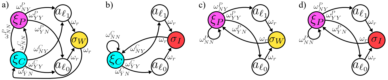
Fig. 2. The policies for the campus patrol robot domain generated for each version of AVE. These policies are illustrated as FSCs, where a circle denotes a controller node labeled with the action taken at that controller node and an arrow denotes a deterministic transition from one controller node to another controller node upon receiving the observation \omega . Note that, in some policies, the observations \omega_{Y^P}^P or \omega_{Y^C}^C , indicating two simultaneous incidents of the same severity at different locations, can deterministically transition to an arbitrary choice of controller nodes.
