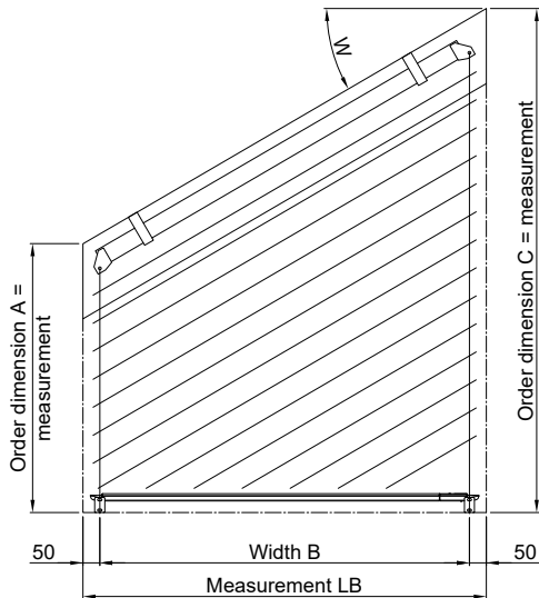
SR1 left Example: Mounting in the reveal
