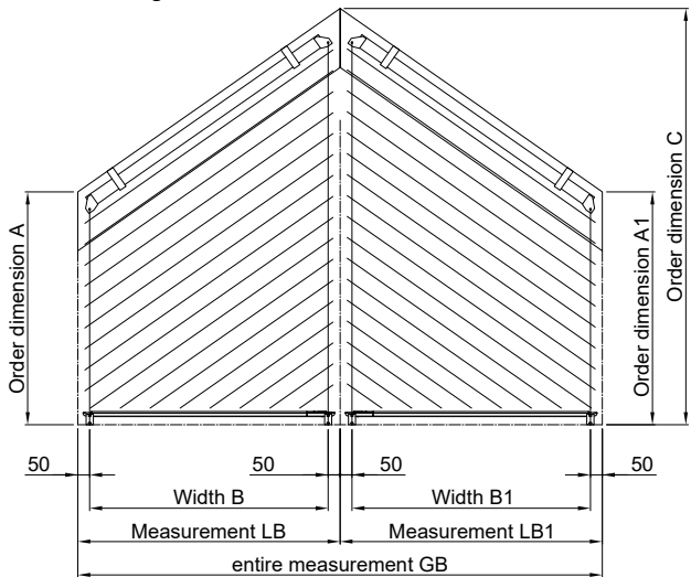
SR7 Example: Mounting in the reveal
