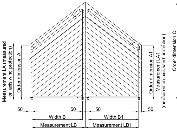
SR7 Example: Mounting in front of the reveal
