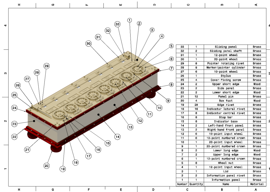
Figure 2. Assembly plan for the Pascaline (Elements 1–33).
