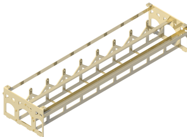
Figure 14. Structure of the assembled Pascaline.
