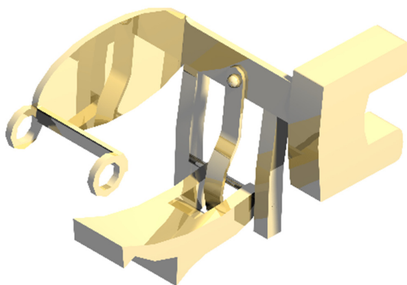
Figure 11. Carry mechanism.
