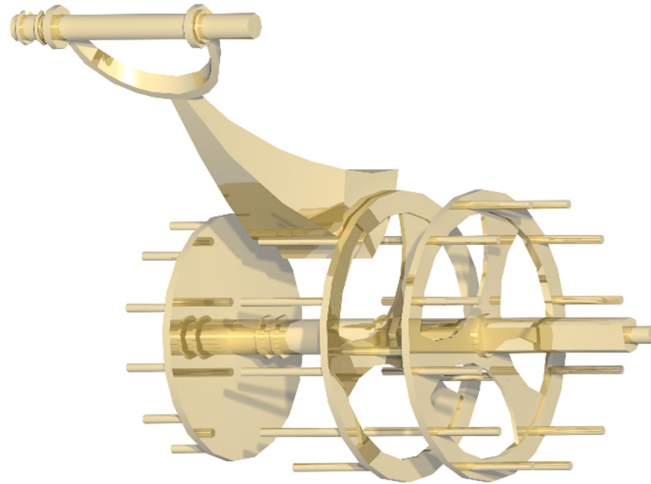
Figure 13. Backstop pawl resting on the accumulator.
