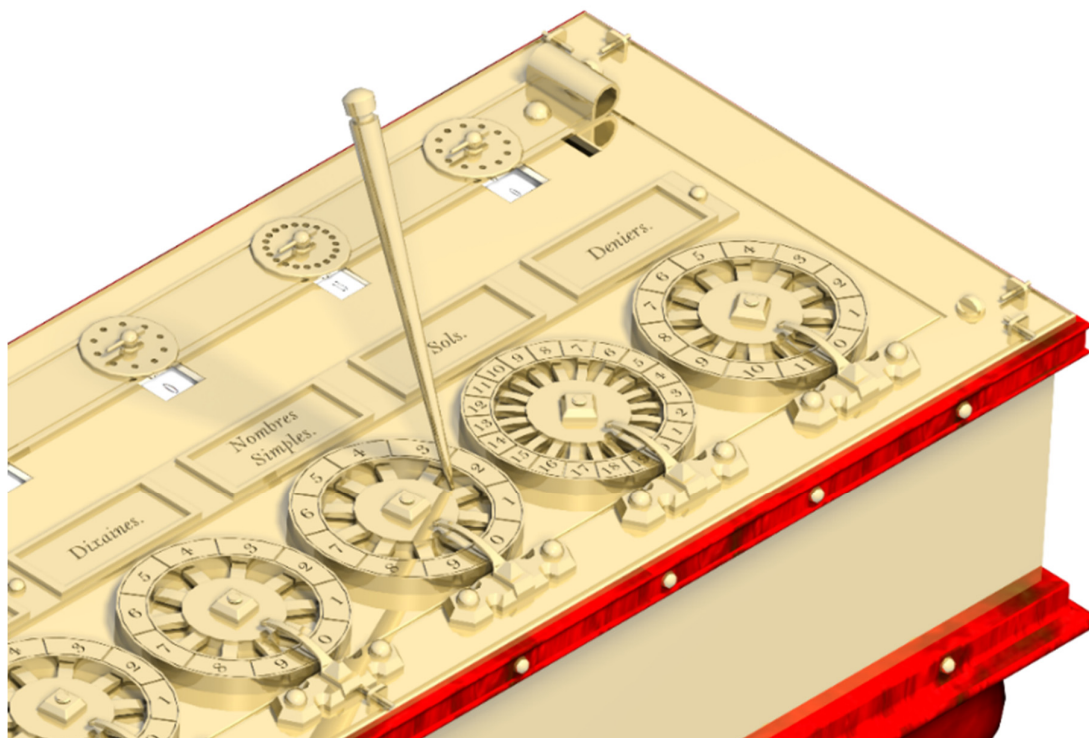
Figure 5. Addend input method.
