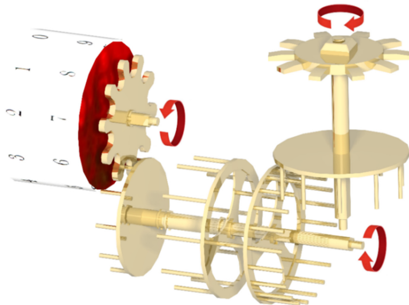
Figure 10. Transmission of the main movement.
