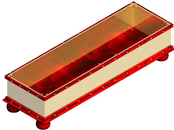
Figure 17. Assembled panels, base, edges and feet.
