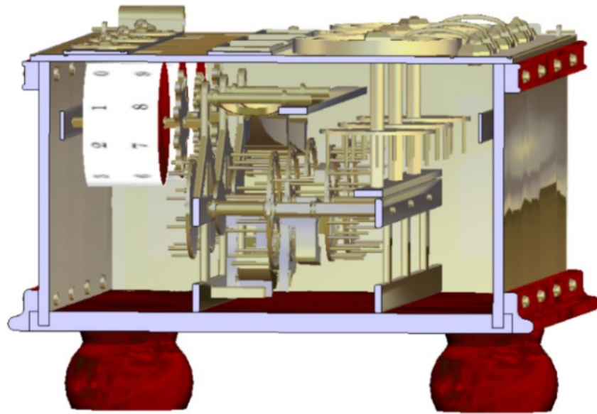
Figure 27. Perspective of the sectioned model.
