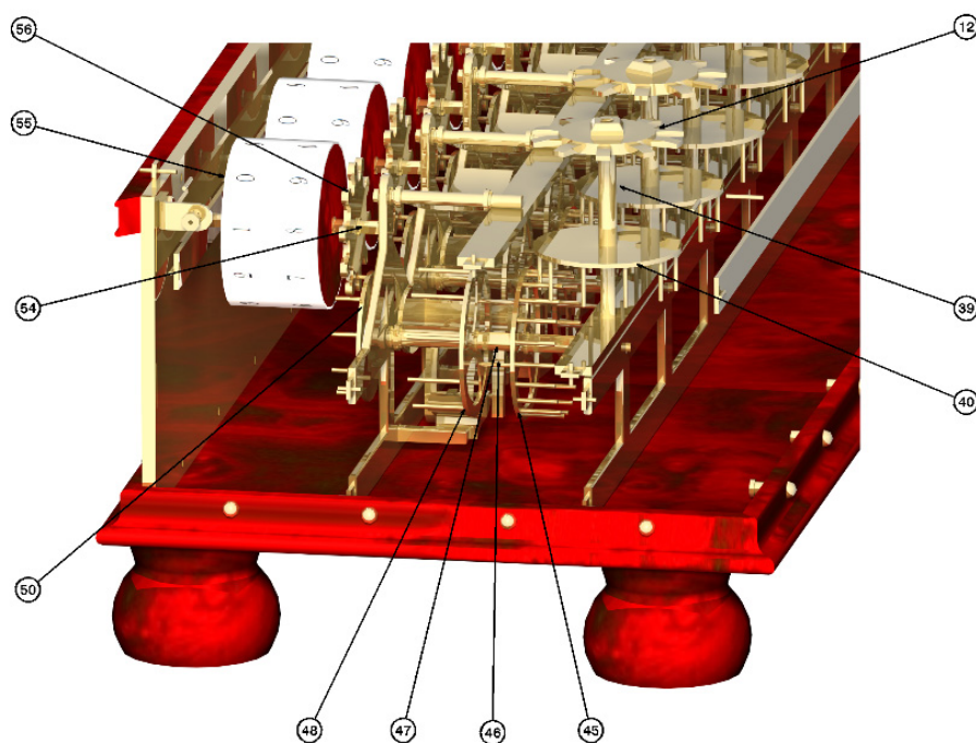
Figure 6. Zoomed representation of the mechanism showed in Figure 3.
